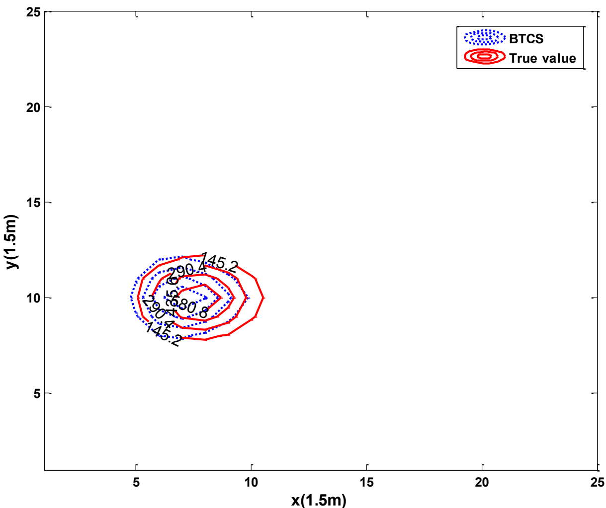
Figure 4.1. Comparison of numerical results and true value at time step 10.
