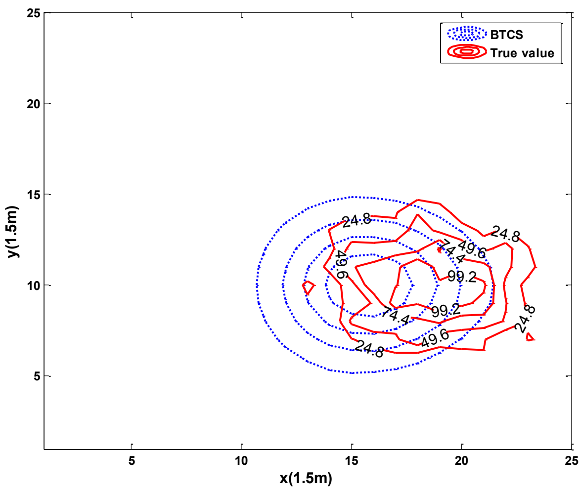
Figure 4.3. Comparison of numerical results and true value at time step 50.
