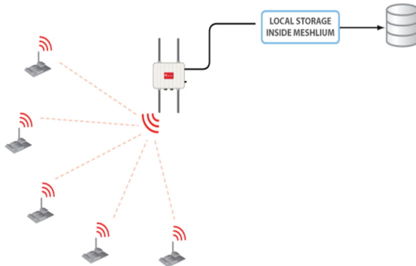
Figure 12 WSN architecture
