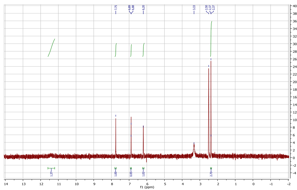
Figure ^1\text{H} NMR spectra of 6-chloro-7-hydroxy-4-methylcoumarin.
