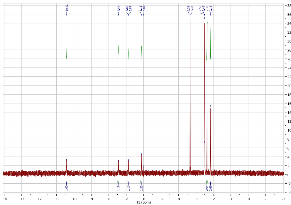
Figure. ^1\text{H} NMR spectra of 7-hydroxy-4,8-dimethylcoumarin.
