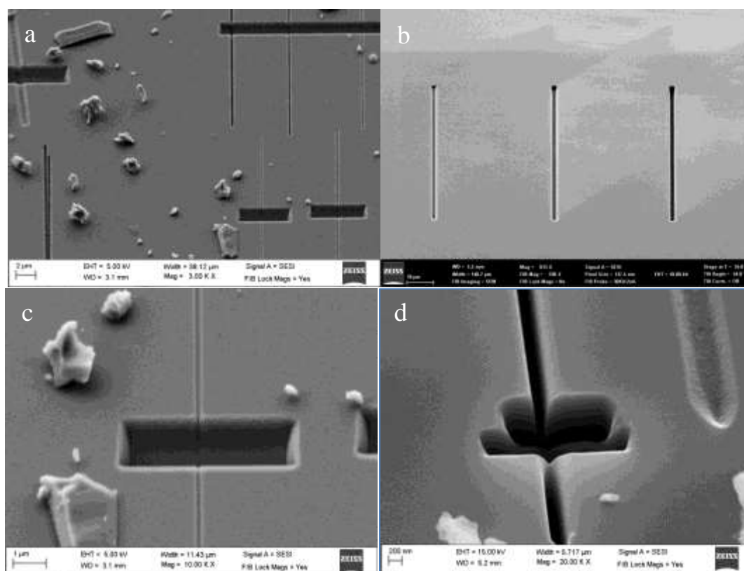
Figure 3.5. Optimization to find clear cut lines: a) Lines in various currents and dosages; b) 2\text{ nA} current with 5\text{nC} , 10\text{nC} and 15\text{ nC} dosage from left to right; c) Observation of depth of a vertical line; d) Milling to find the width of the vertical line.
