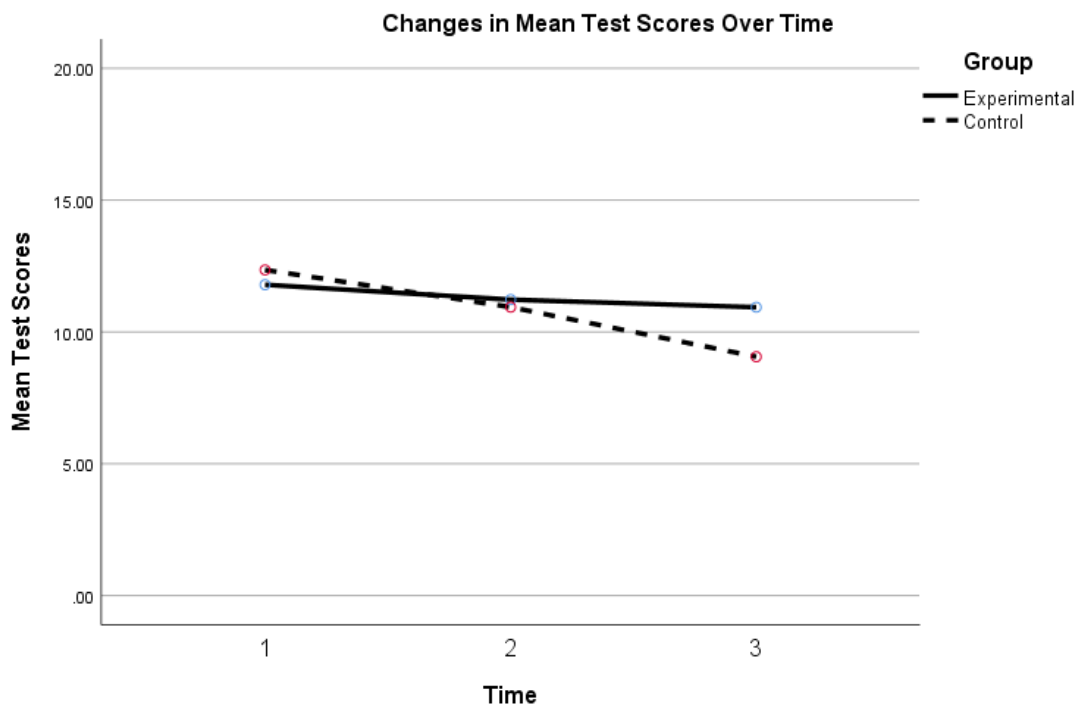
Figure 2. Changes in both groups' mean test scores over time.
