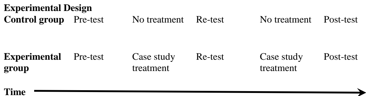
Figure 1. Quasi-experimental repeated measures design adapted from Creswell (2014, p. 310).
