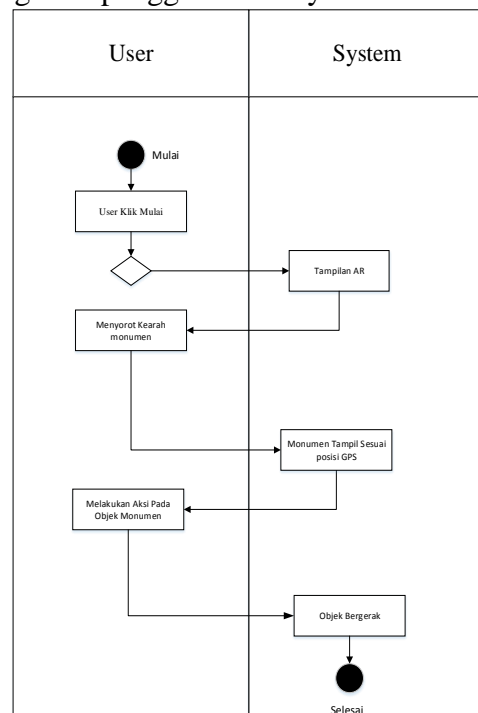
Gambar 3. Activity Diagram
