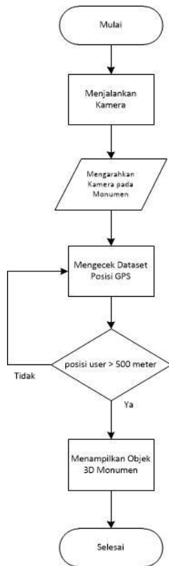
Gambar 4. Flowchart
