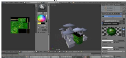
Gambar 6. Objek 3D
