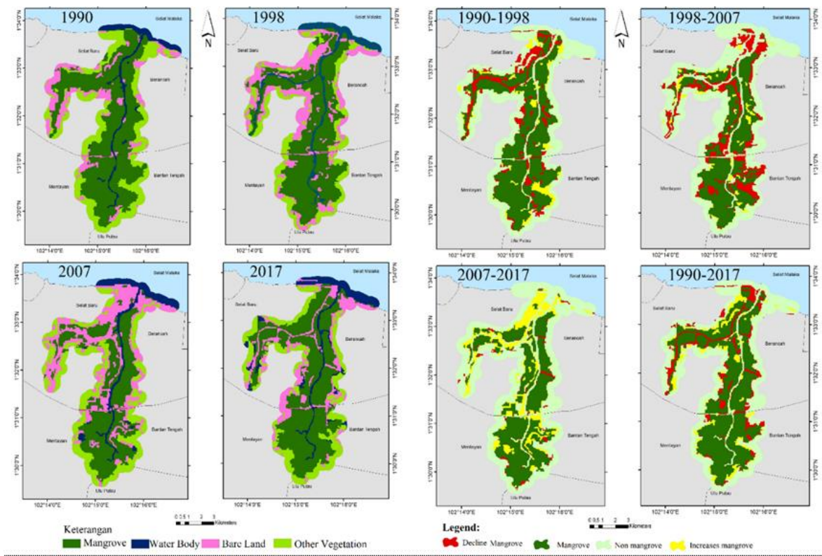
Fig 2. (a) Classification of land cover mangrove (b) Mangrove change (1990-2017)
