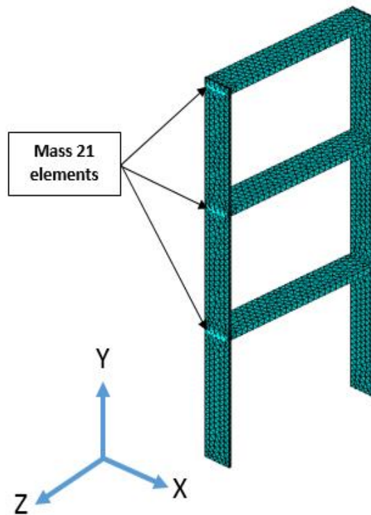
Figure 10: Discretisation of model, mass addition and coordinate system.
