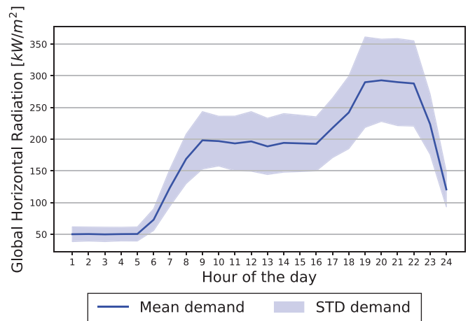
Figure 3: Daily average electrical demand
