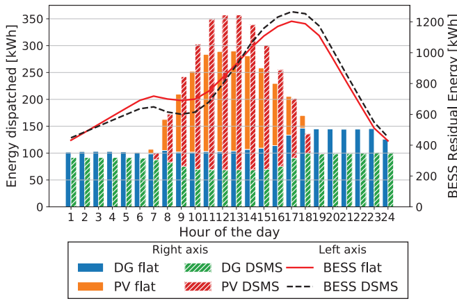
Figure 10: Daily average dispatch before and after the application of the DSMS
