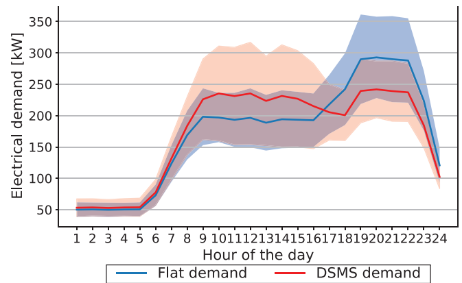
Figure 9: Comparison of the electrical demand before and after the application of the DSMS
