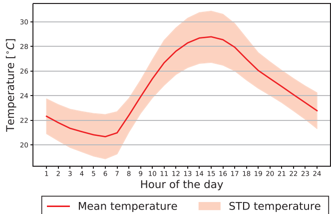
Figure 5: Daily average temperature
