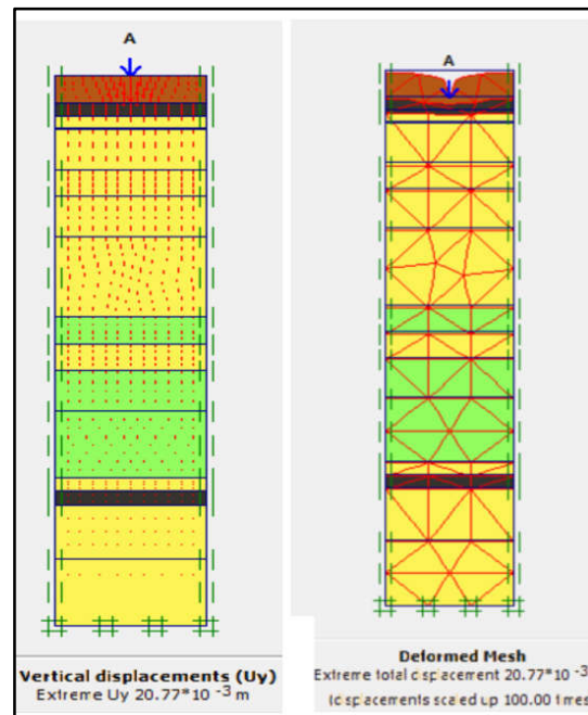
Fig. 6. Plaxis Modeling On Declining Soil.
