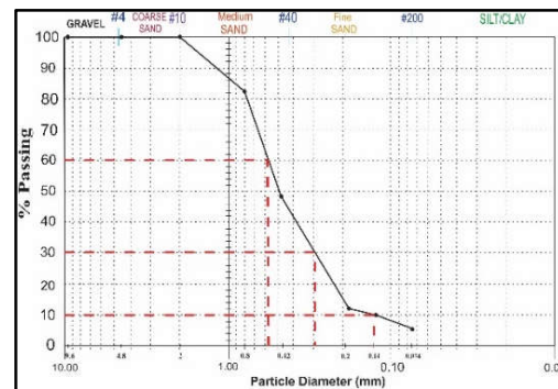
Fig. 3. Graph Sieve analysis on Drill Sample 1 (8.00-8.50) M.
