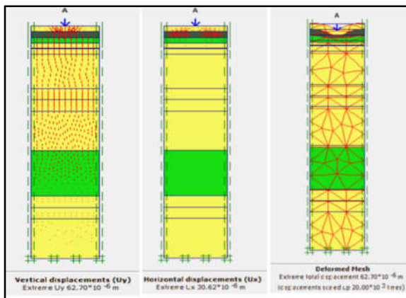
Fig. 5. Plaxis Modeling Power Capacity To Support Land.
