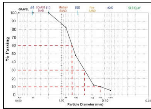
Fig. 4. Graph Sieve analysis on Drill Sample 3 (8.00-8.50) M.
