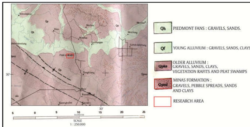
Fig. 1. Regional Geological Map of research Area.
