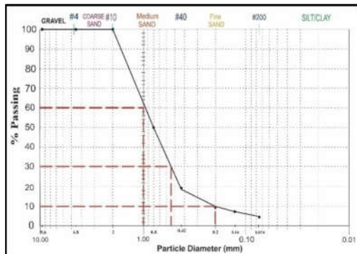
Fig. 2. Graph Sieve analysis on Drill Sample 1 (4.50-5.00) M.
