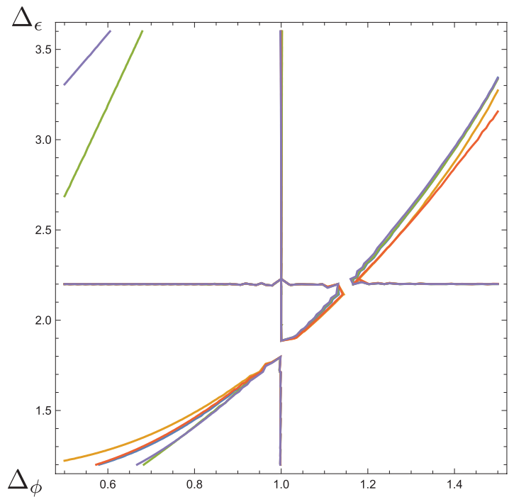
Fig. 13. D = 4.0 (global map): the contours of zero loci of minors are shown with Q = 6.0 , \Delta_1 = 2.2 . The fixed point (Gaussian) \Delta_\epsilon = 2.0 , \Delta_\phi = 1.0 is on the line \Delta_\phi = 1.0 .
