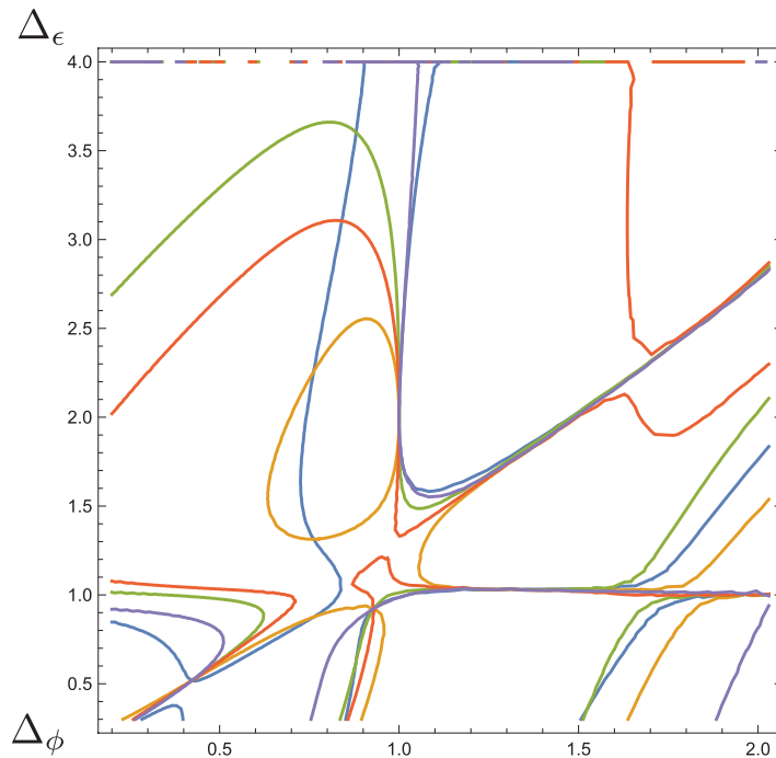
Fig. 2. Yang–Lee in D = 4 : The zero loci of 4 \times 4 minors intersect at three fixed points. The free-field fixed point for \phi^4 theory at \Delta_\phi = 1, \Delta_\epsilon = 2 is shown as an intersection point of the five minor loci. The lower fixed point corresponds to the Yang–Lee edge singularity (\Delta_\epsilon = \Delta_\phi = 0.8) . The parameters Q = 6.0 and \Delta_{\epsilon'} = 4.0 are chosen.
