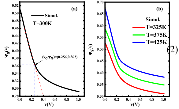
Figure. 4. Surface potential-forward voltage curves of the Au/InSb/InP Schottky diode
