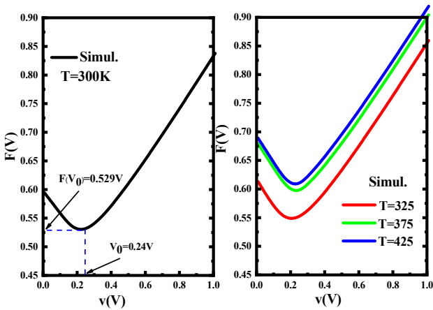
Figure.3. F(V) as a function of V obtained from forward bias current-voltage characteristics of the Au/InSb/InP Schottky diode (a) at T=300K and (b) for T=(325, 375 and 425K)
