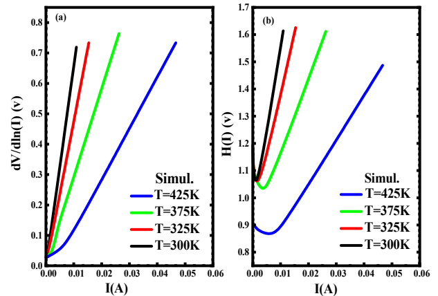
Figure.2. the obtained of \left(\frac{dV}{d(\ln(I))}\right) and H(I) as a function of ( I ) for Au/InSb/InP Schottky diode, at different temperatures
