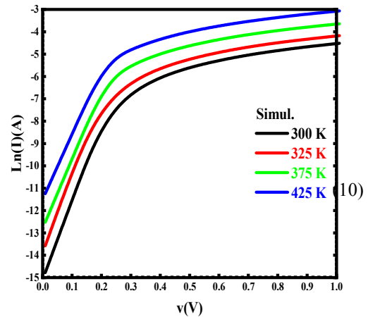
Figure .1. The (I-V) characteristics of Au/InSb/InP Schottky diode in the temperature range (300–425 K).
