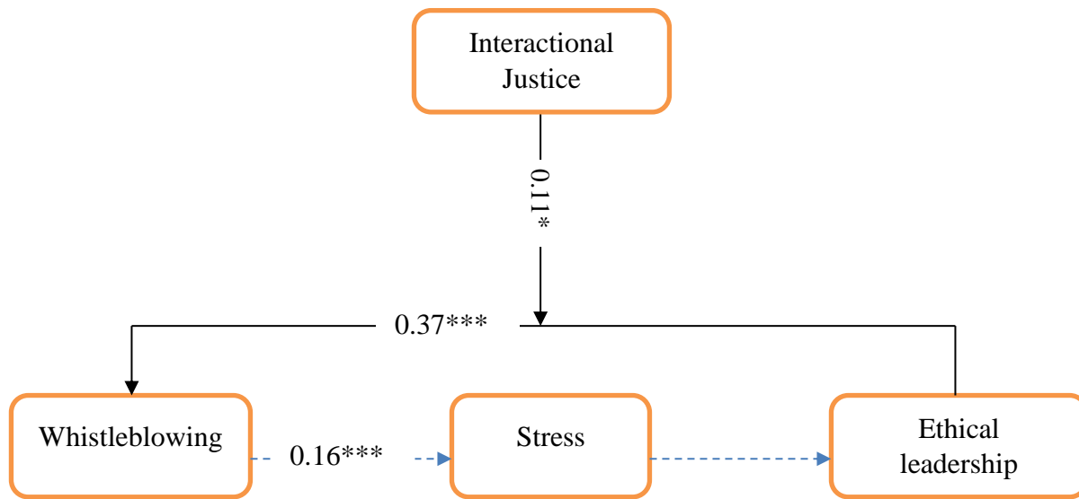
Figure 1 - Hypothesized Framework
