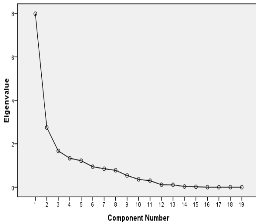
Scree Plot
