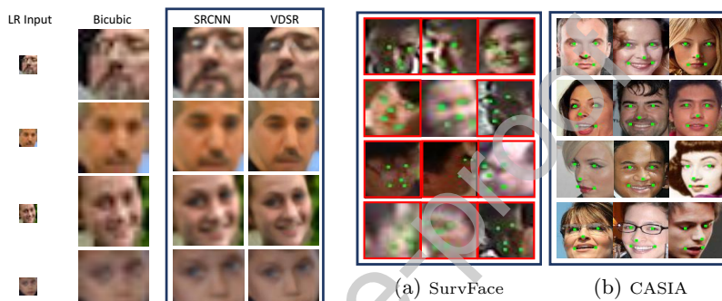
Figure 10: Super-resolved MegaFace2 images. CentreFace is used jointly with the super-resolution models. Figure 11: Facial landmark detection [112] on (a) SurvFace and (b) CASIA web faces. Red box: failure cases.
