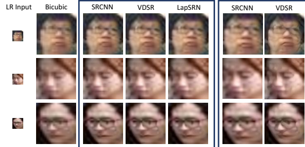
Figure 8: Super-resolved images on SurvFace by independently ( left box ) and jointly ( right box ) trained super-resolution models. CentreFace is used in joint training.
