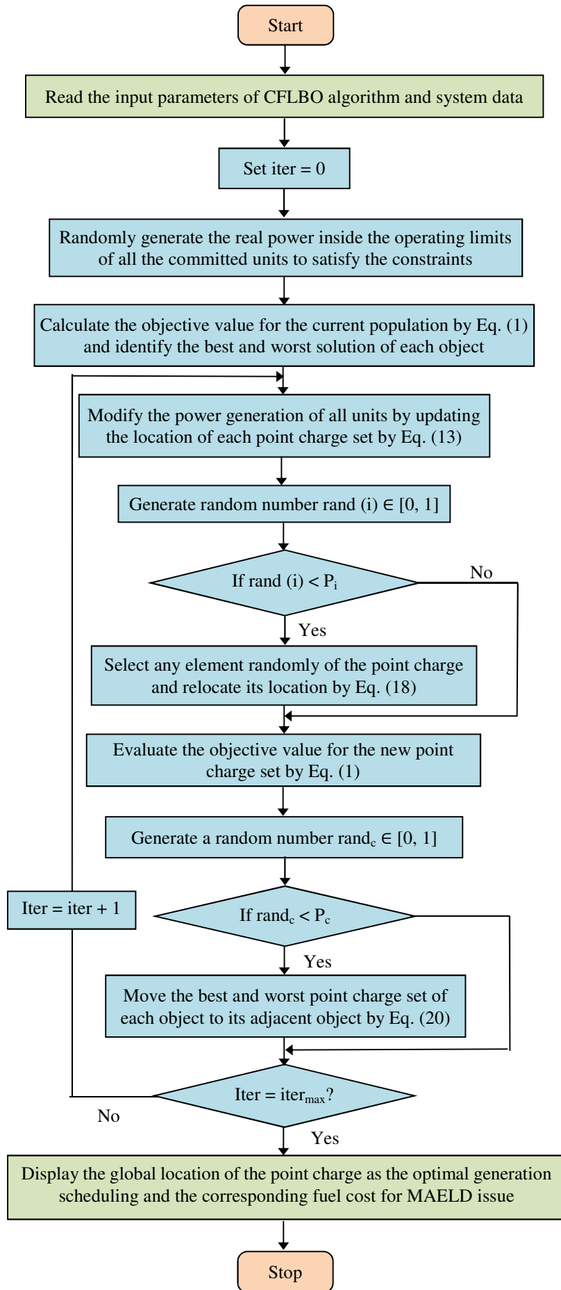
Fig. 2 Flow chart of CFLBO approach applied in MAELD issues
