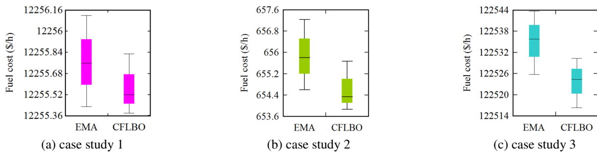
Fig. 11 Box-Whisker plot for the obtained fuel costs in 50 runs
