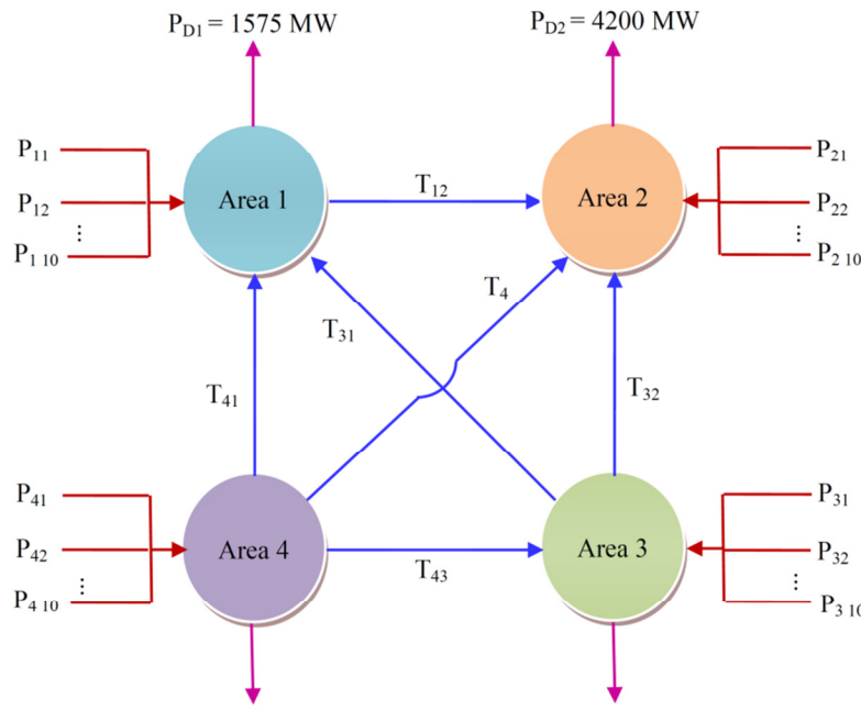
Fig. 7 Schematic diagram of four-area system
