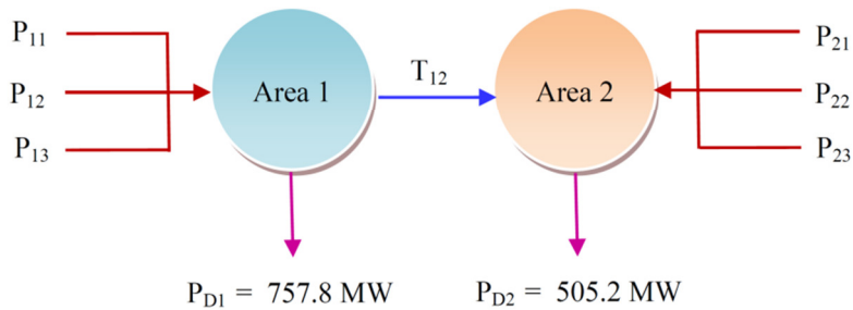
Fig. 3 Schematic diagram of two-area system
