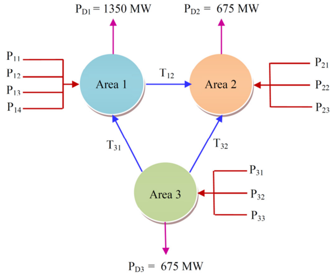
Fig. 5 Schematic diagram of three-area system
