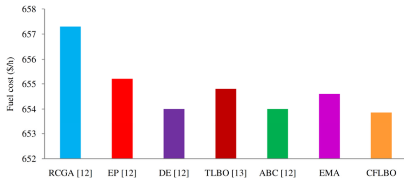
Fig. 6 Comparison of generation costs incurred by various approaches for case study 2
