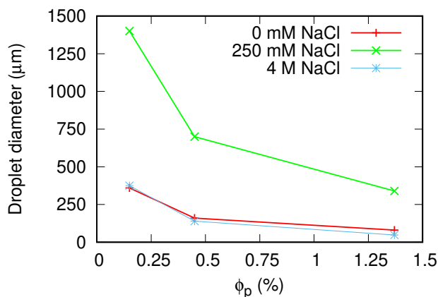
Fig. 5 – NaCl Volume-weighted median droplet size at different [\text{NaCl}] and particle volume fractions, \phi_p . Measurements were made using light scattering, except for the lower two \phi_p at [\text{NaCl}] = 250 mM, which were estimated from photographs. All samples had \Phi_{\text{IM}} = 0\% and were emulsified using a vortex mixer for 30 s each.
