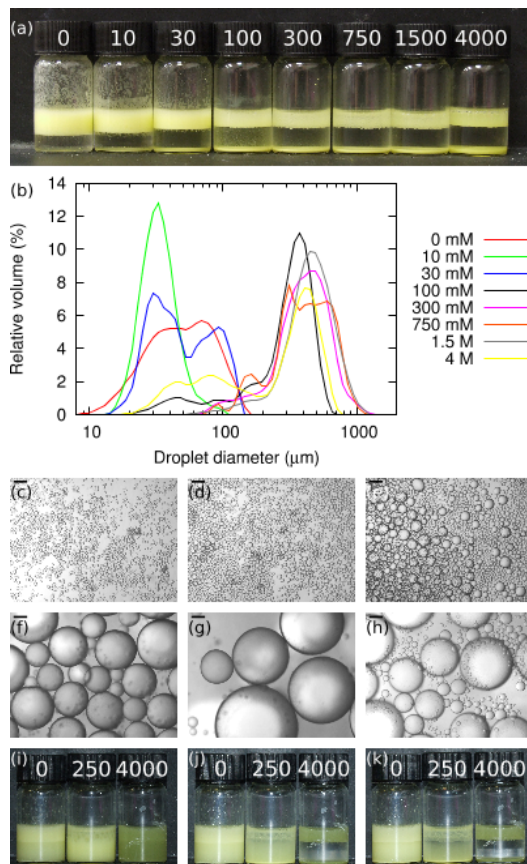
Fig. 2 – NaCl (a) Photograph showing emulsions stabilised by Stöber silica (yellow due to FITC dye) at various sodium chloride concentrations (on vial, mM). The amount of free silica at the base of the vial increases with salt concentration. (b) Size distributions of emulsions at various sodium chloride concentrations. In all samples, \phi_p = 1.7\% , \phi_o = 20\% and \Phi_{IM} = 10\% . (c-h) Micrographs of emulsions at sodium chloride concentrations of 0 mM, 10 mM, 30 mM, 100 mM, 300 mM and 4000 mM. The scale bars are 100 \mu\text{m} . (i-k) Photographs of emulsions at salt concentrations shown on each vial, mM. In all three samples \phi_p = 1.1\% , \phi_o = 20\% and \Phi_{IM} = 0\% . The times since emulsification are 0, 40 and 80 min.
