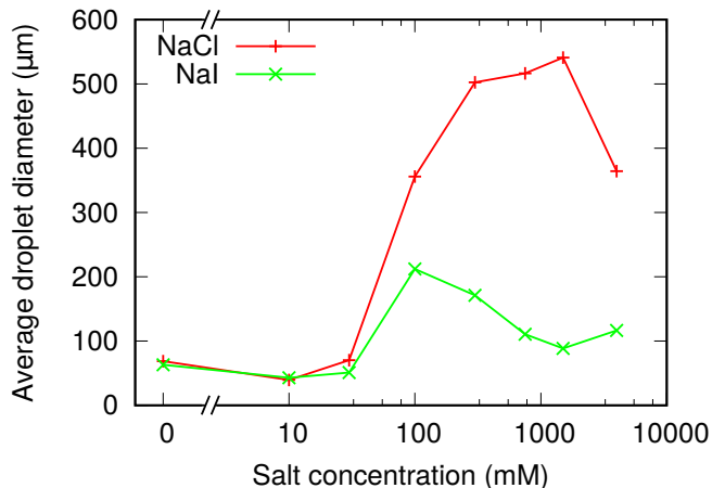
Fig. 3 – NaCl & NaI: Volume-weighted mean droplet size of emulsions at different sodium chloride and sodium iodide concentrations. In all samples, \phi_p = 1.7\% , \phi_o = 20\% and \Phi_{IM} = 10\% .
