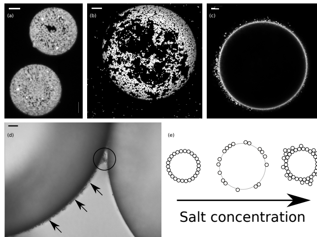
Fig. 4 – NaCl (a) Confocal micrograph z-projection of 14 images, with a z-spacing of 0.44 \mu\text{m} (ImageJ 21 ) showing the particle layers at two droplet interfaces. [\text{NaCl}] = 10 mM; the scale bar is 5 \mu\text{m} . (b) Confocal micrograph z-projection of 42 images, with a z-spacing of 0.44 \mu\text{m} showing the packing of particles at the interface. [\text{NaCl}] = 30 mM; the scale bar is 20 \mu\text{m} . (c) Confocal micrograph showing the thickened particle layer at the interface in the 100 mM sample. The scale bar is 20 \mu\text{m} . (d) Micrograph showing the thickening of the interfacial particle layer. The arrows indicate the thickened particle layer, which protrudes several micrometres into the continuous phase and the circled area shows that the layer can be shared by droplets. [\text{NaCl}] = 300 mM; the scale bar is 10 \mu\text{m} . (e) Cartoon summarizing the behaviour of droplets as the salt concentration is increased, see text.
