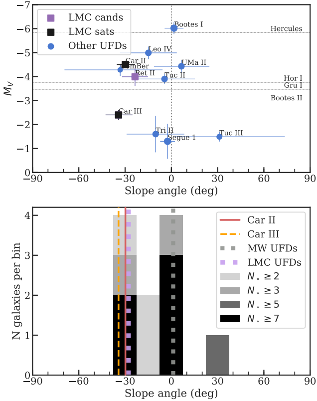
Figure 7. Top: [\text{Mg}/\text{Ca}] vs [\text{Fe}/\text{H}] slope angles for all UFDs vs luminosity M_V . Slope error bars indicate 68% posterior region, and measurements with smaller uncertainties have correspondingly larger symbols. The luminosities of galaxies with unconstrained slope posteriors are shown as horizontal lines. Square symbols indicate UFDs that are LMC satellites (Car II, Car III, Hor I) or satellite candidates (Ret II). Round symbols indicate UFDs likely associated with the Milky Way. Bottom: histogram of [\text{Mg}/\text{Ca}] slope angles for all UFDs. UFDs with more stars (i.e., more confident slope measurements) are shown as darker shades of grey. The relatively extreme slope angles for Car II and III are marked as vertical solid and dashed lines, respectively. The total [\text{Mg}/\text{Ca}] slopes for all MW vs LMC UFD stars are marked in dotted grey and purple lines, respectively.
