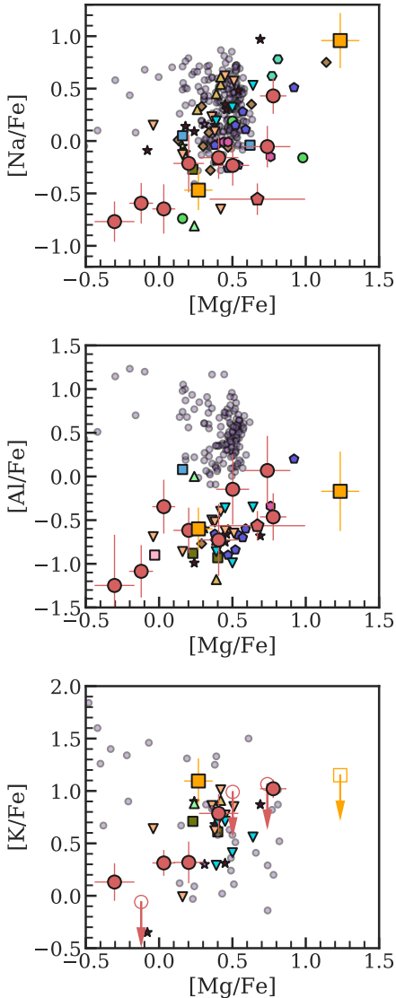
Figure 5. Mg-Na, Mg-Al, and Mg-K abundance patterns. Car II is red circles/pentagon, Car III is orange squares, globular cluster stars are small purple circles, and other UFDs are small colored points (same as Figure 2). In globular clusters, Mg-Na and Mg-Al are anti -correlated, while in both Car II and Car III these elements are clearly correlated. Mg-K are anticorrelated in the globular cluster NGC 2419, and there is no evidence for such in Car II. The light element correlations confirm that Car II and III are dwarf galaxies and not globular clusters.
