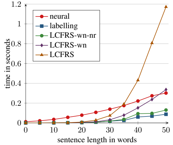
Figure 2: Parsing speed on Negra.
