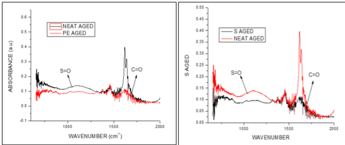
(a) Neat and PE modified bitumen
