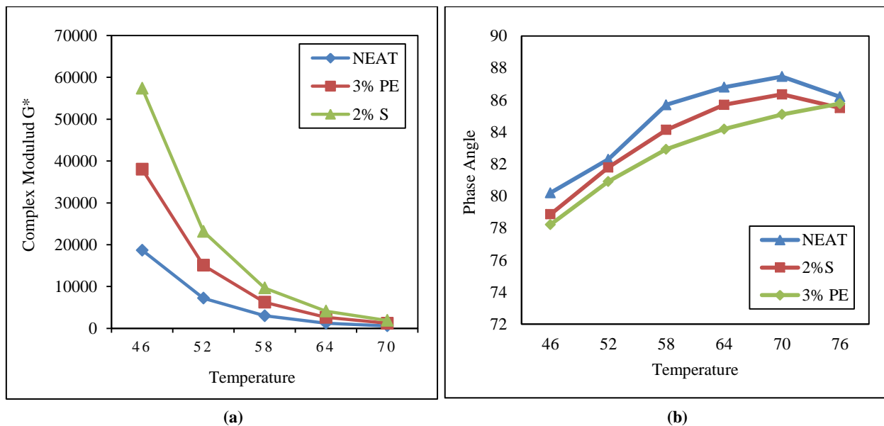
Figure 16. Variation of (a) Complex Modulus and (b) Phase angle of Neat and Modified bitumen before aging
