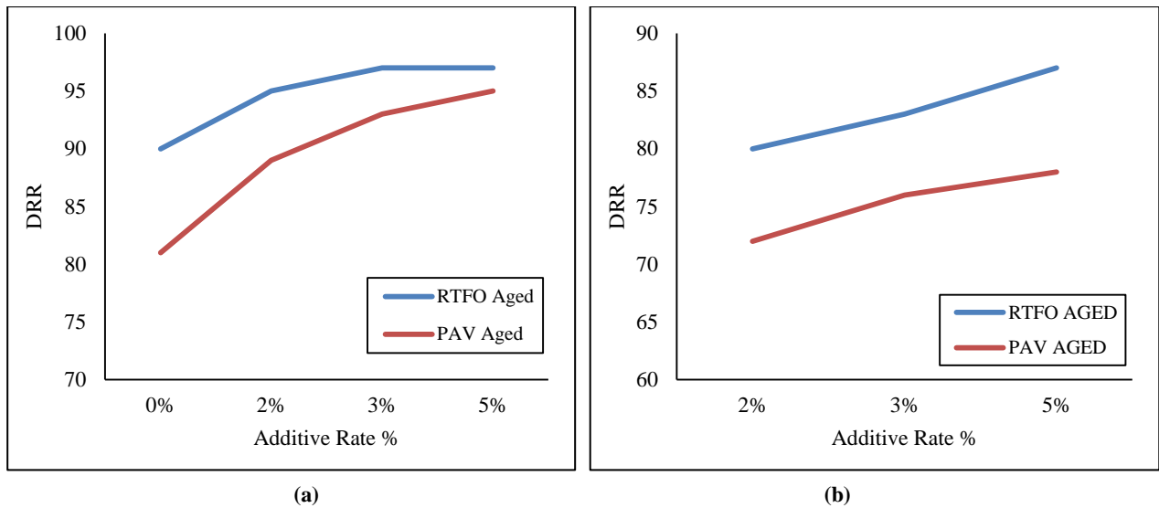
Figure 11. Ductility Retained Ratio for (a) Polyethylene modified bitumen and (b) Sulphur modified bitumen
