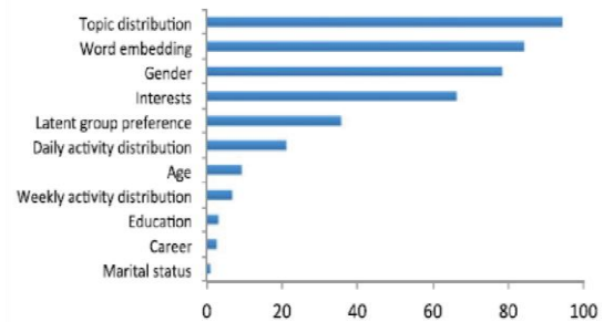
Fig.2. Relative attribute importance ranking (corresponding to the features)
