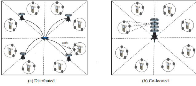
Fig. 1. Distributed and co-located mm-Wave massive MU-MIMO systems.
