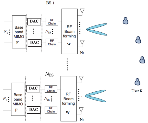
Fig. 2. Hardware impaired distributed MIMO transmitter based-hybrid beamforming structure.
