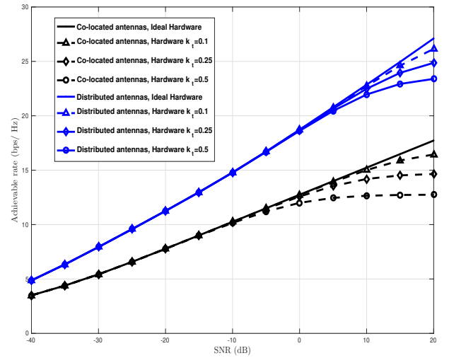
Fig. 3. Performance comparison of distributed and co-located mm-Wave massive MU-MIMO systems with different levels of impairments.
