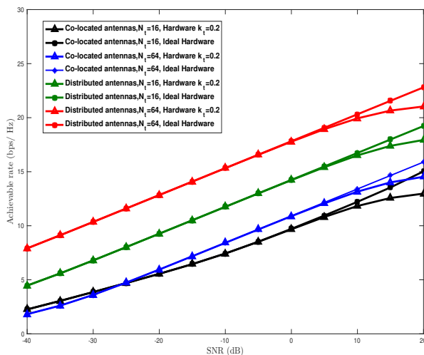
Fig. 4. Achievable rate performance comparison of distributed and co-located mm-Wave massive MU-MIMO systems with different antennas configurations.
