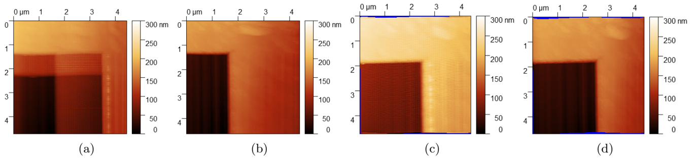
Figure 8. Region of an orthogonal grating. Images generated with x - y data taken from (a) piezo driving voltage signals, trace and retrace in both axes (b) voltage signals, trace only in both axes (c) interferometer signals, trace and retrace in both axes (d) interferometer signals, trace only in both axes. z data is the same for all images. Blue regions (at the top of images c and d) represent blank space due to non-straight image edges. Note that the hysteresis associated with the piezos leads to both ghosting of trace and retrace and spurious curvature, problems both of which have been eliminated by the real-time interferometer measurements.
