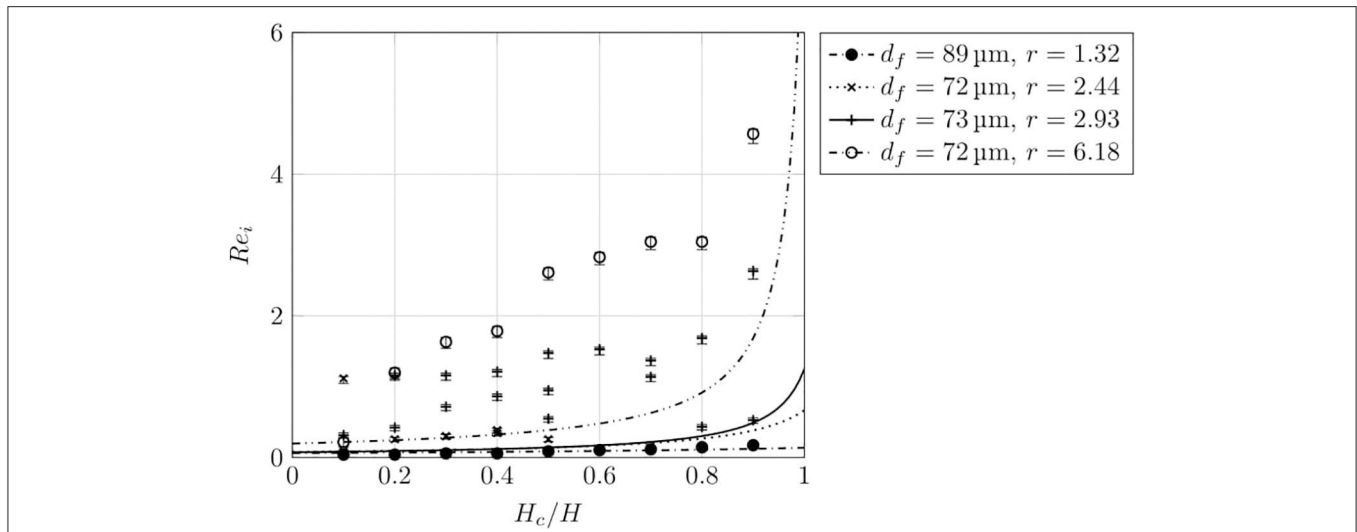
FIGURE 9 | Dependence of initiation Reynolds number on relative coarse layer thickness for several beds consisting of mixtures of particles as specified in Table 2 . All the beds had an overall thickness H = 10 cm. The curves describe Equation 10 and the points are experimental measurements.
