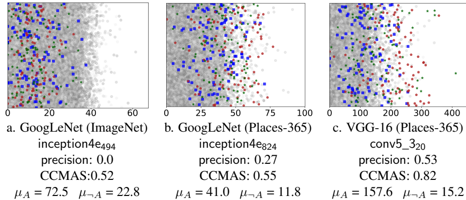
Figure 6: The units with with the highest Network Dissection scores for the category ‘bus’. The scatter plots, precision, and CCMAS scores all indicate a low selectivity for this category. blue squares: ‘school bus’; red pentagons: ‘trolleybus’; green stars: ‘minibus’; grey circles: other classes.
