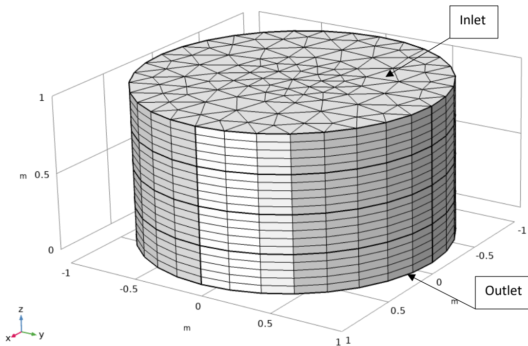
Figure 8: Mesh of the computer model representing a portion of the shipbreaking yard.
