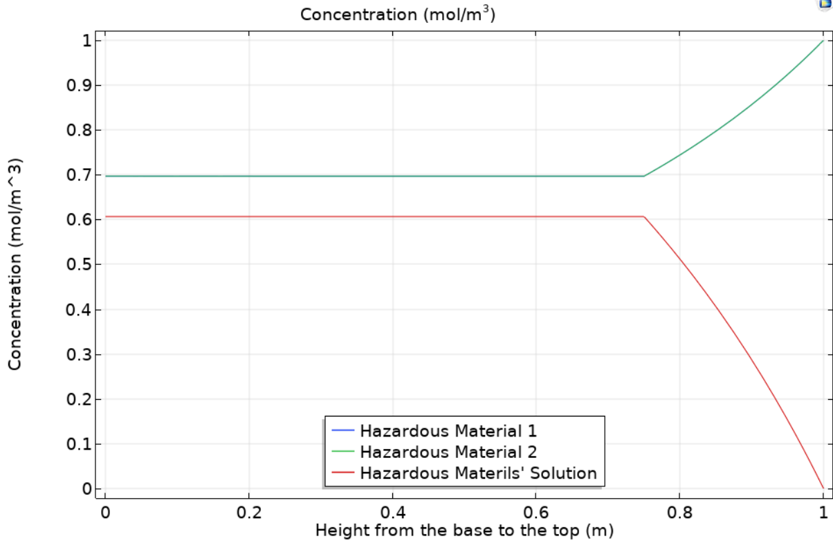
Figure 11: Plot of concentration of hazardous materials and the solution product across the depth of the yard ground at 1.0 atmospheric pressure.
