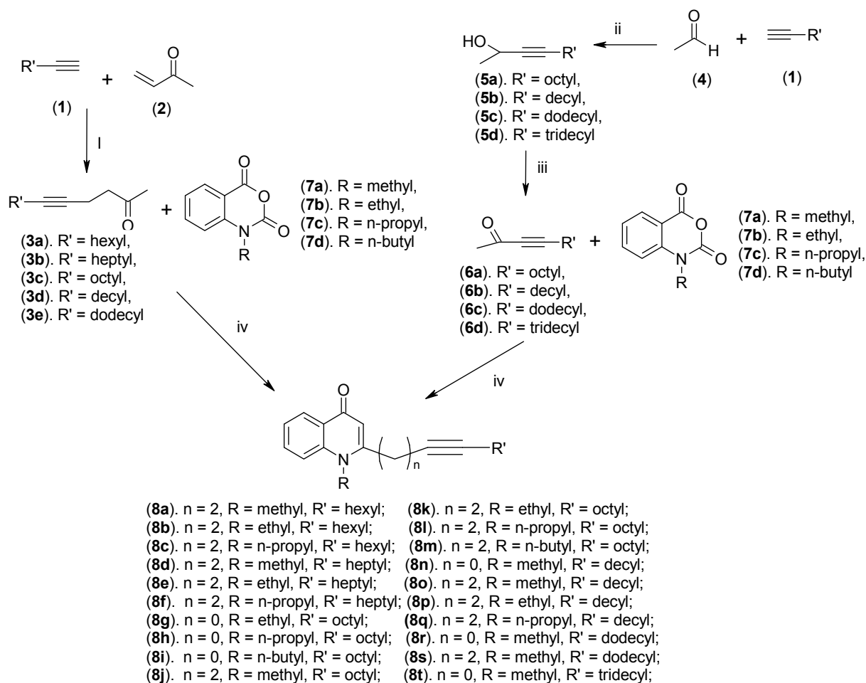
Scheme 1. Synthesis of N -alkyl-2-alkynyl-4(1 H )-quinolones.
