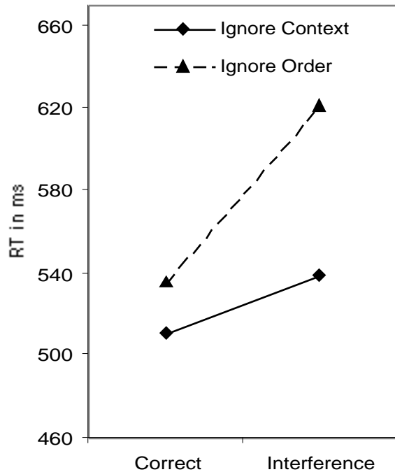
Figure 7: RTs with and without interfering violation.
