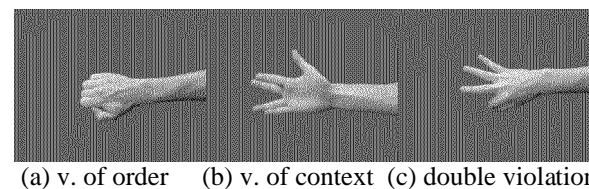
Figure 5: Examples for violation of order, context, and double violation in Experiment 2.
