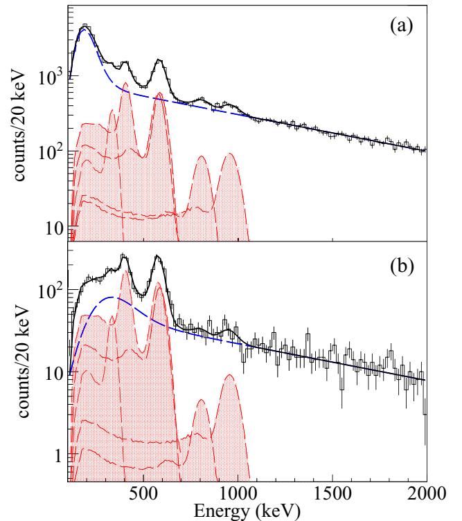
FIG. 2. (a) Doppler-shift corrected \gamma -ray spectrum from inelastic scattering of ^{136}\text{Te} on the C target. The fit to the experimental spectrum is shown as a thick black line which is the sum of the background (blue dashed line) and the simulated DALI2 response for \gamma rays with energies of 353, 423, 607, 810, and 962 keV (red dashed lines). No cut on the \gamma -ray multiplicity was applied. (b) Same as (a), but for the one-neutron transfer reaction \text{C}(^{137}\text{Te}, ^{136}\text{Te}) . Here, only events with multiplicity M_\gamma < 4 are considered. In both parts of the figure add-back was applied.
