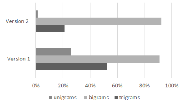
Figure 6: Segmenter performance with unigram, bigram, and trigram models.
