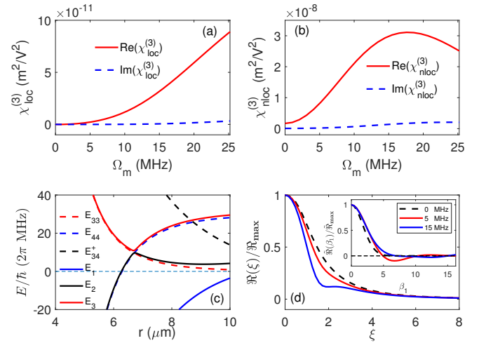
FIG. 2. Kerr nonlinearity enhancement, interaction potential energy, and normalized nonlinear response function \Re of the probe field in the presence of the microwave dressing. (a) Real part \text{Re}(\chi_{\text{loc}}^{(3)}) (solid red line) and imaginary part \text{Im}(\chi_{\text{loc}}^{(3)}) (dotted blue line) of the local nonlinear susceptibility \chi_{\text{loc}}^{(3)} as a function of the half Rabi frequency \Omega_m of the microwave field. (b) The same as (a) but for the nonlocal nonlinear susceptibility \chi_{\text{nloc}}^{(3)} . (c) Potential-energy curves E_1 (solid blue line), E_2 (solid black line), and E_3 (solid red line) of two Rydberg atoms as functions of the interatomic distance r = |\mathbf{r}' - \mathbf{r}| for \Omega_m = 10 MHz and \Delta = 13.98 MHz; E_{33} (dashed blue line), E_{44} (dashed black line), and E_{34}^+ (dashed red line) are for the case without the microwave field. (d) Normalized response function \Re/\Re_{\text{max}} as a function of the dimensionless coordinate \xi = x/R_0 ( R_0 is the typical transverse beam radius of the probe field) with \Omega_m = 0 (dotted black line), 5 MHz (solid red line), and 15 MHz (solid blue line), respectively. Inset: the normalized response function \Re/\Re_{\text{max}} in momentum space (i.e. the Fourier transformation of \Re/\Re_{\text{max}} ) as a function of the dimensionless wavenumber \beta_1 = R_0 k_x ( k_x is the dimensional wavenumber in x direction) with \Omega_m = 0, 5, \text{ and } 15 MHz, respectively.
