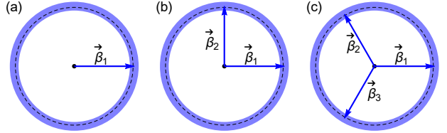
FIG. 7. Schematic diagram of the non-dimensional wavevectors \vec{\beta}_j for different optical self-organized structures. (a) Parallel stripes; (b) Square lattice, for which \vec{\beta}_1 \cdot \vec{\beta}_2 = 0 ; (c) Hexagonal lattice, for which \vec{\beta}_1 + \vec{\beta}_2 + \vec{\beta}_3 = 0 . All the wavevectors have the same module (i.e. |\vec{\beta}_j| \approx \beta_{\text{cr}} ; \beta_{\text{cr}} is the first wavenumber of the unstable band of the MI).
