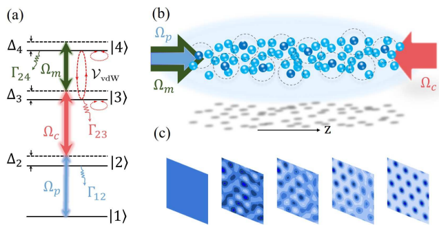
FIG. 1. Schematics of the model. (a) Ladder-type four-level atomic configuration for realizing the microwave-dressed Rydberg-EIT. Here, the weak probe laser field (blue), strong control laser field (red), and strong microwave field (green) with half Rabi frequencies \Omega_p , \Omega_c , and \Omega_m drive the transitions |1\rangle \leftrightarrow |2\rangle , |2\rangle \leftrightarrow |3\rangle , and |3\rangle \leftrightarrow |4\rangle , respectively; States |1\rangle and |2\rangle are respectively ground and excited states, both |3\rangle and |4\rangle are highly excited Rydberg states; \Delta_2 , \Delta_3 , and \Delta_4 are respectively the one-, two-, and three-photon detunings; \Gamma_{12} , \Gamma_{23} , and \Gamma_{24} are the spontaneous emission decay rates from |2\rangle to |1\rangle , |3\rangle to |2\rangle and |4\rangle to |2\rangle , respectively. Two Rydberg atoms locating respectively at position \mathbf{r} and \mathbf{r}' interact through van der Waals potential \hbar V_{\text{vdw}}^l(\mathbf{r}' - \mathbf{r}) ( l = s, d, e ; see text). (b) Possible experimental geometry, where small solid circles denote atoms and large dashed circles denote Rydberg blockade spheres. (c) Emergence of an optical pattern via modulation instability.
