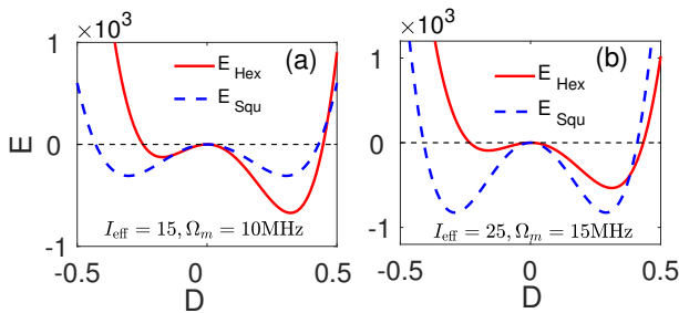
FIG. 8. Ground-state energy for cases of hexagonal and square lattices. (a) Ground-state energy E as a function of modulation amplitude D , with parameters \beta_{\text{cr}} = 4.3 , I_{\text{eff}} = 15 , \Omega_m = 10 MHz, and \sigma = 1 . The solid red line ( E_{\text{Hex}} ) is for the hexagonal pattern; the dotted blue line ( E_{\text{Squ}} ) is for the square pattern. (b) The same as (a) but for \beta_{\text{cr}} = 4.3 , I_{\text{eff}} = 25 , \Omega_m = 15 MHz, and \sigma = 1 .
