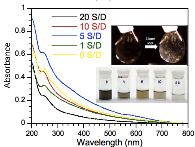
Figure 1. UV-Vis spectra of rGO(1) solutions after various exposures. Insets: top : drop suspension before (left) and after (right) several laser shots (the Teflon tube above the drop is 1.6 mm in diameter); bottom : Graphene solutions before (left) and after laser irradiation (532 nm laser, 45 mJ/pulse).
