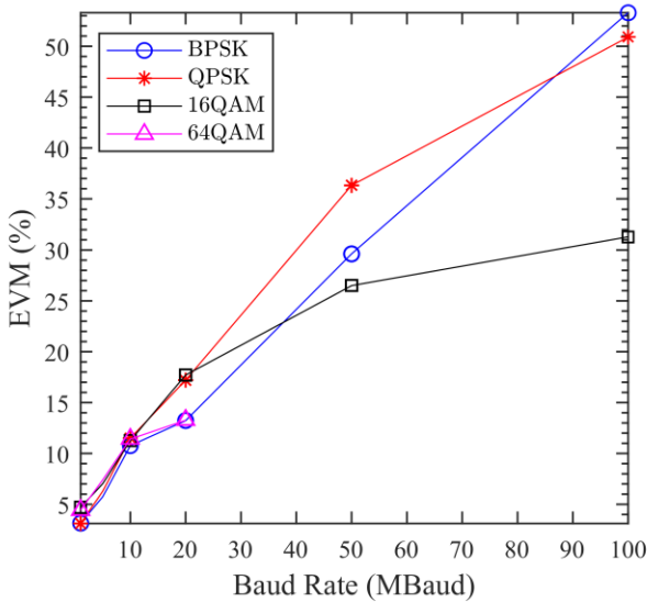
Fig. 7: Measured EVM of mmW link over 2 m experimental setup for different digital modulation schemes link (Section III.C: hybrid VLC/mmW antenna implementation in a real system).
