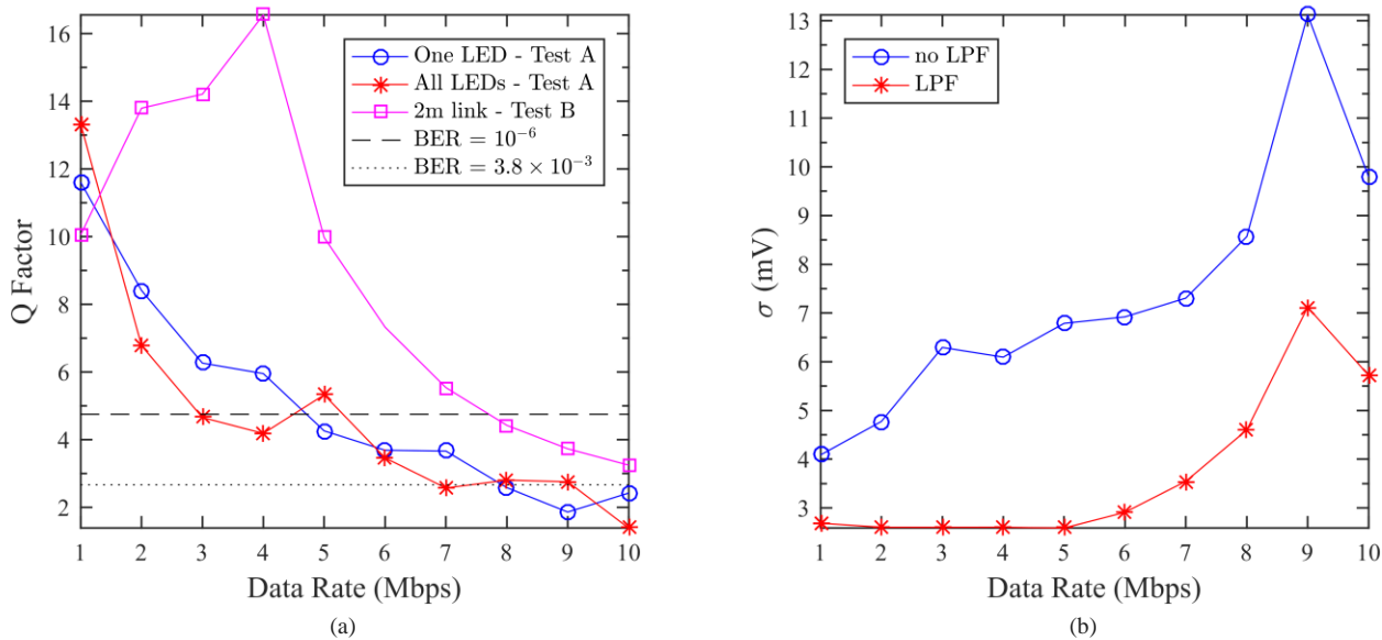
Fig. 5: (a) The Q-factor as a function of the data rate for the hybrid antenna with a single LED and all LEDs (Section III.B: VLC test) and for the BER values of 3.8 \times 10^{-3} and 10^{-6} . Also shown is the performance of VLC Tx over a 2 m link (Section III.C: hybrid VLC/mmW antenna implementation in a real system). (b) Standard deviation versus the data rate for the Rx output voltage before and after LPF (Section III.B: VLC test).
