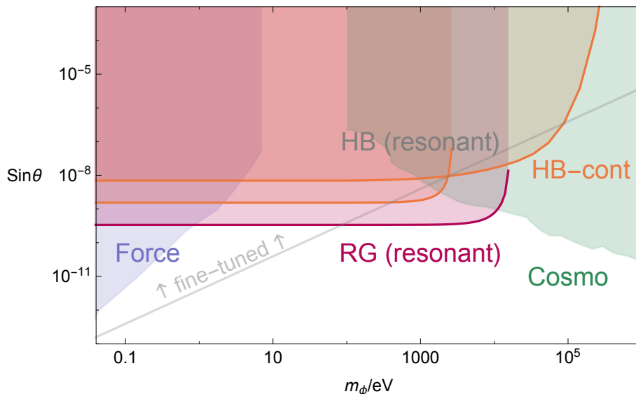
Figure 6. Constraints on a scalar \phi with a Higgs portal coupling (section 3.4.3), where \sin\theta is the mixing with the SM Higgs. Force bounds [32–36] are in blue, stellar cooling bounds (see text) in red and orange, and cosmological constraints in green. The latter arise from a freeze-in relic abundance decaying around the present day, contributing to the observed photon background [44] (we show these bounds as extending up to couplings at which \phi would decay at BBN time, though it would require further work to verify whether the constraints are valid there). Since most of the nucleon mass comes from QCD, rather than from the Higgs VEV, the ratio of nucleon to electron \phi couplings is smaller than the nucleon-electron mass ratio. The electron coupling therefore dominates the \phi -SM mixing, and thus the resonant \phi production, as well as dominating the continuum production. The stellar cooling bounds are therefore the appropriate rescaling of the \phi\bar{e}e bounds show in the left-hand panel of figure 5, and likewise continue to very small \phi masses. The grey line shows the approximate fine-tuning bound \sin\theta \lesssim m_\phi/v_{EW} [45], demonstrating that our new stellar constraints are able to probe natural parameter space.
