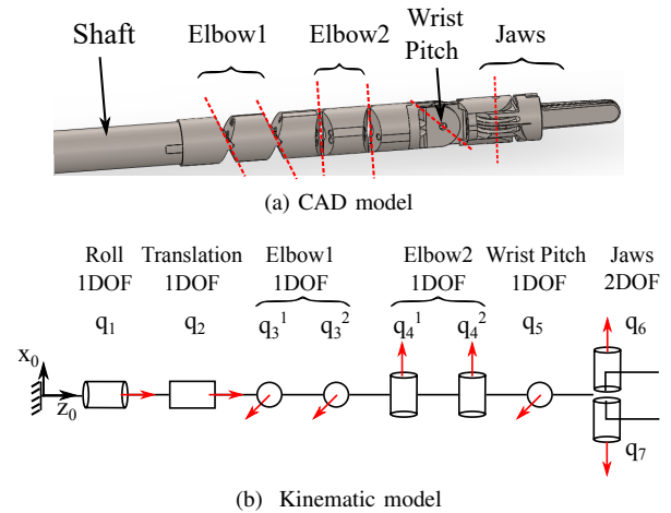
Fig. 2: Micro-IGES surgical tool: 2a) CAD model; 2b) kinematic model
