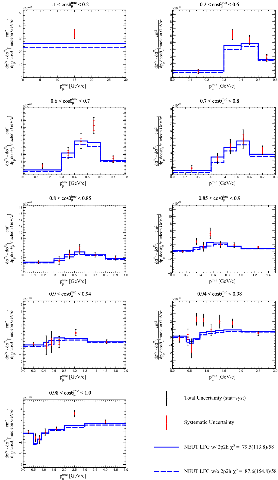
FIG. 18. Measured double-differential \nu_{\mu}-\bar{\nu}_{\mu} CC- 0\pi cross section difference in bins of true muon kinematics with systematic uncertainty (red bars) and total (stat. + syst.) uncertainty (black bars). The results are compared to NEUT version 5.4.1, which uses an LFG + RPA model, with (solid line) and without (dashed line) 2p2h. The full and shape-only (in parenthesis) \chi^2 are reported. The last bin in momentum is not displayed for readability.
