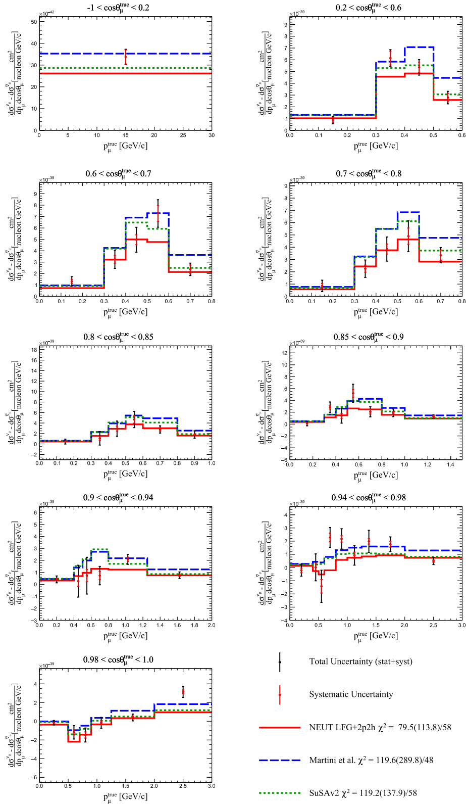
FIG. 23. Measured double-differential \nu_{\mu}-\bar{\nu}_{\mu} CC- 0\pi cross section difference in bins of true muon kinematics with systematic uncertainty (red bars) and total (stat. + syst.) uncertainty (black bars). The results are compared to NEUT version 5.4.1, which uses an LFG + RPA model with 2p2h (solid red line), Martini et al. (dashed blue line) and SUSAV2 (green dashed line) models. The full and shape-only (in parenthesis) \chi^2 are reported. The last bin in momentum is not displayed for readability.
