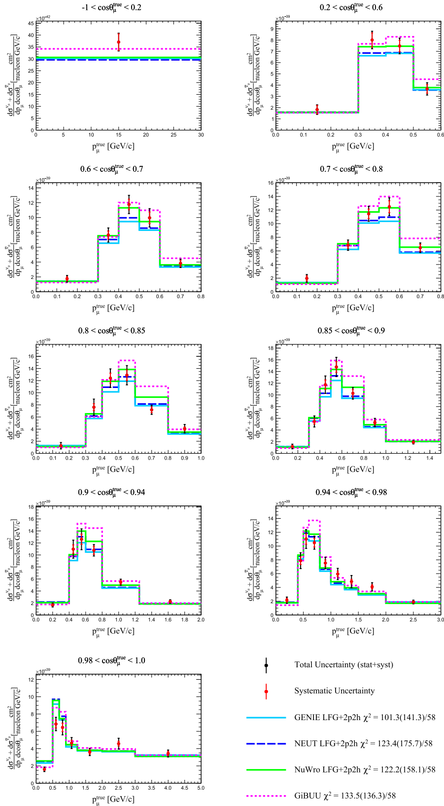
FIG. 27. Measured double-differential \nu_{\mu} + \bar{\nu}_{\mu} CC- 0\pi cross section sum in bins of true muon kinematics with systematic uncertainty (red bars) and total (stat. + syst.) uncertainty (black bars). The result is compared with NEUT (dashed blue line), NUWRO version 18.02.1 (green solid line) and GiBUU 2019 (pink dotted line) prediction. All generators use an LFG + RPA model that includes 2p2h. The full and shape-only (in parenthesis) \chi^2 are reported. The last bin in momentum is not displayed for readability.
