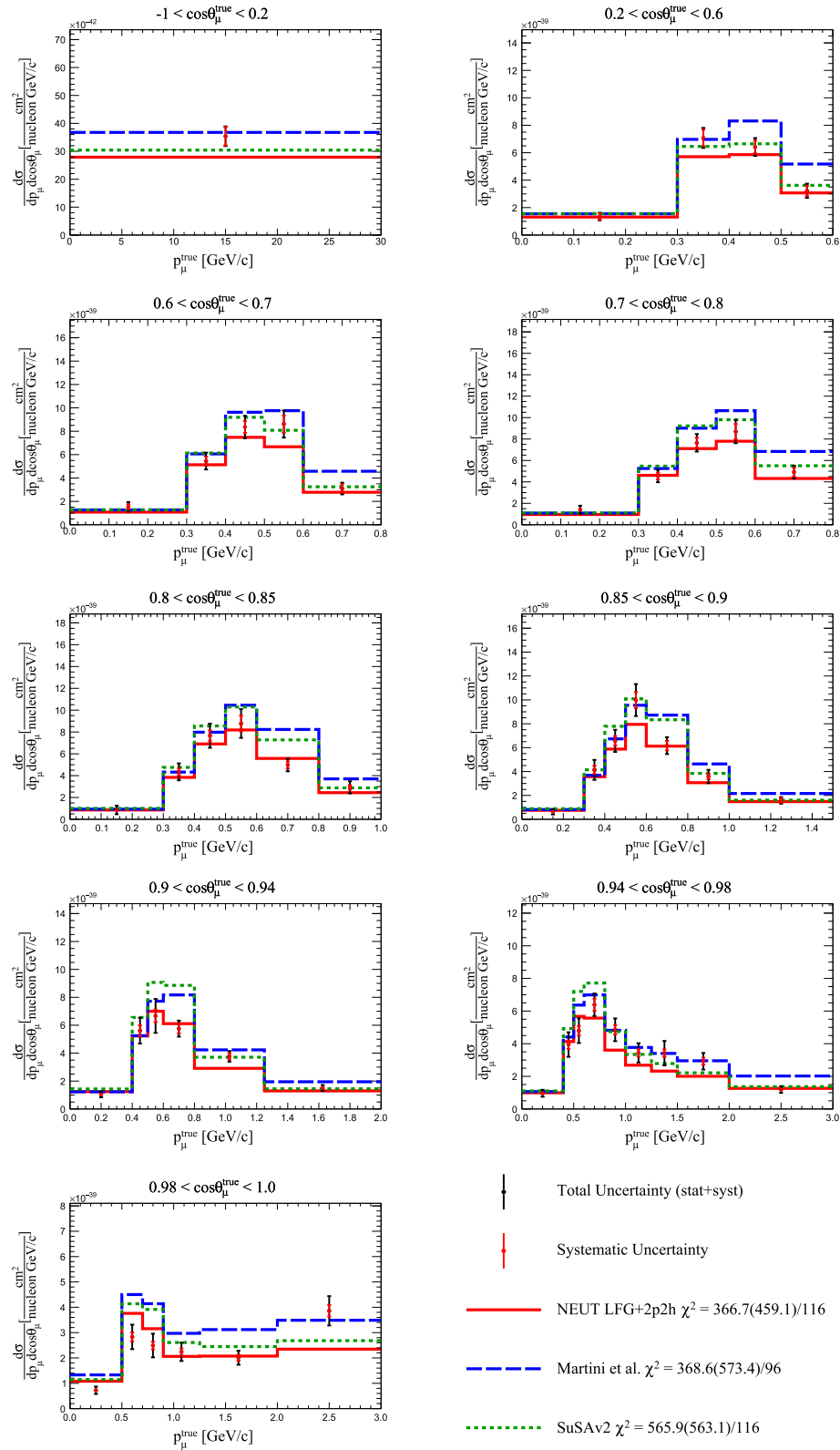
FIG. 20. Measured \nu_{\mu} CC- 0\pi double-differential cross section per nucleon in bins of true muon kinematics with systematic uncertainty (red bars) and total (stat. + syst.) uncertainty (black bars). The results are compared to NEUT version 5.4.1, which uses an LFG + RPA model with 2p2h (solid red line), Martini et al. (dashed blue line) and SUSAV2 (green dashed line) models. The full and shape-only (in parenthesis) \chi^2 are reported. The last bin in momentum is not displayed for readability.
