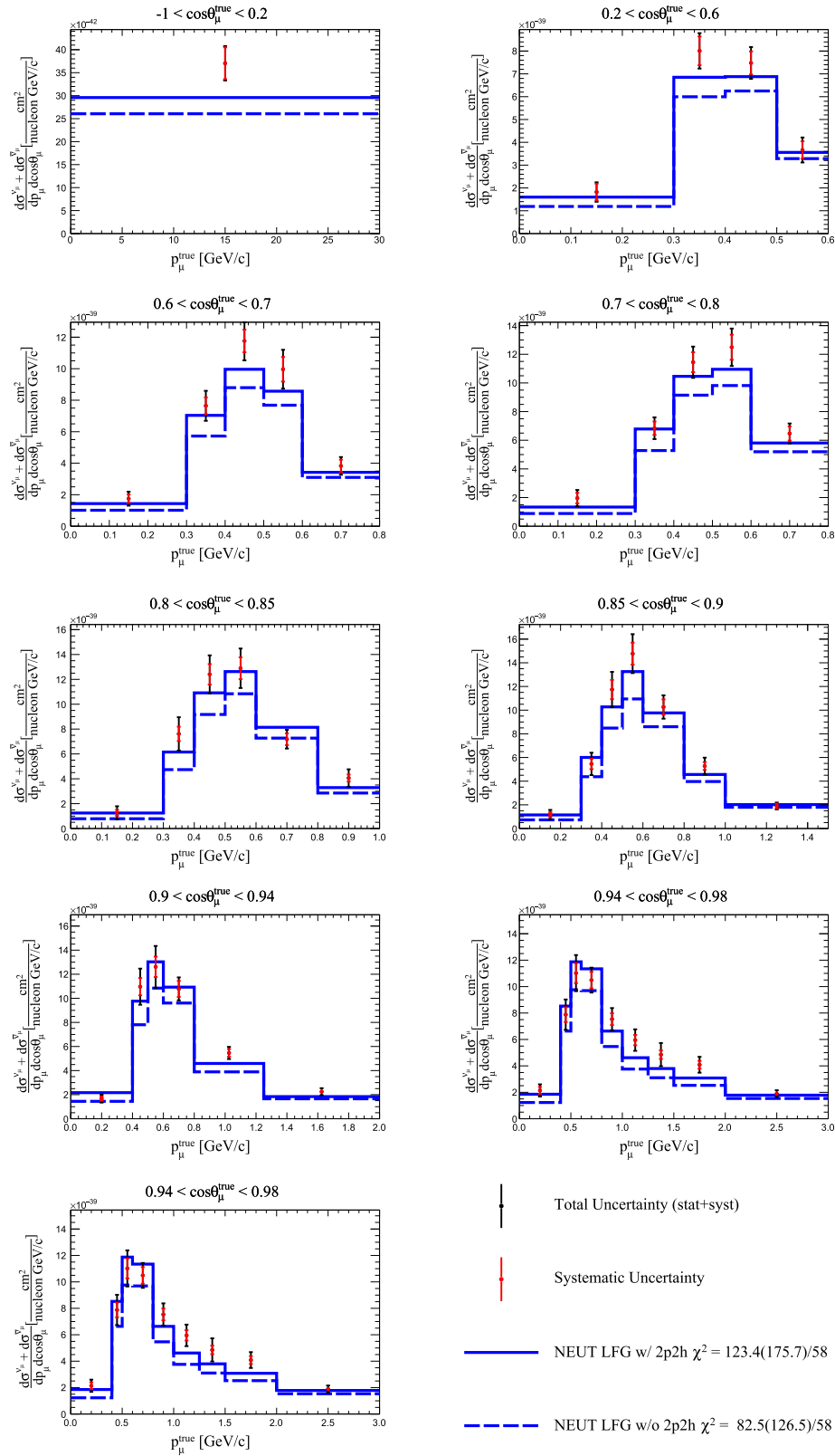
FIG. 17. Measured double-differential \nu_{\mu} + \bar{\nu}_{\mu} CC-0 \pi cross section sum in bins of true muon kinematics with systematic uncertainty (red bars) and total (stat. + syst.) uncertainty (black bars). The results are compared to NEUT version 5.4.1, which uses an LFG + RPA model, with (solid line) and without (dashed line) 2p2h. The full and shape-only (in parenthesis) \chi^2 are reported. The last bin in momentum is not displayed for readability.
