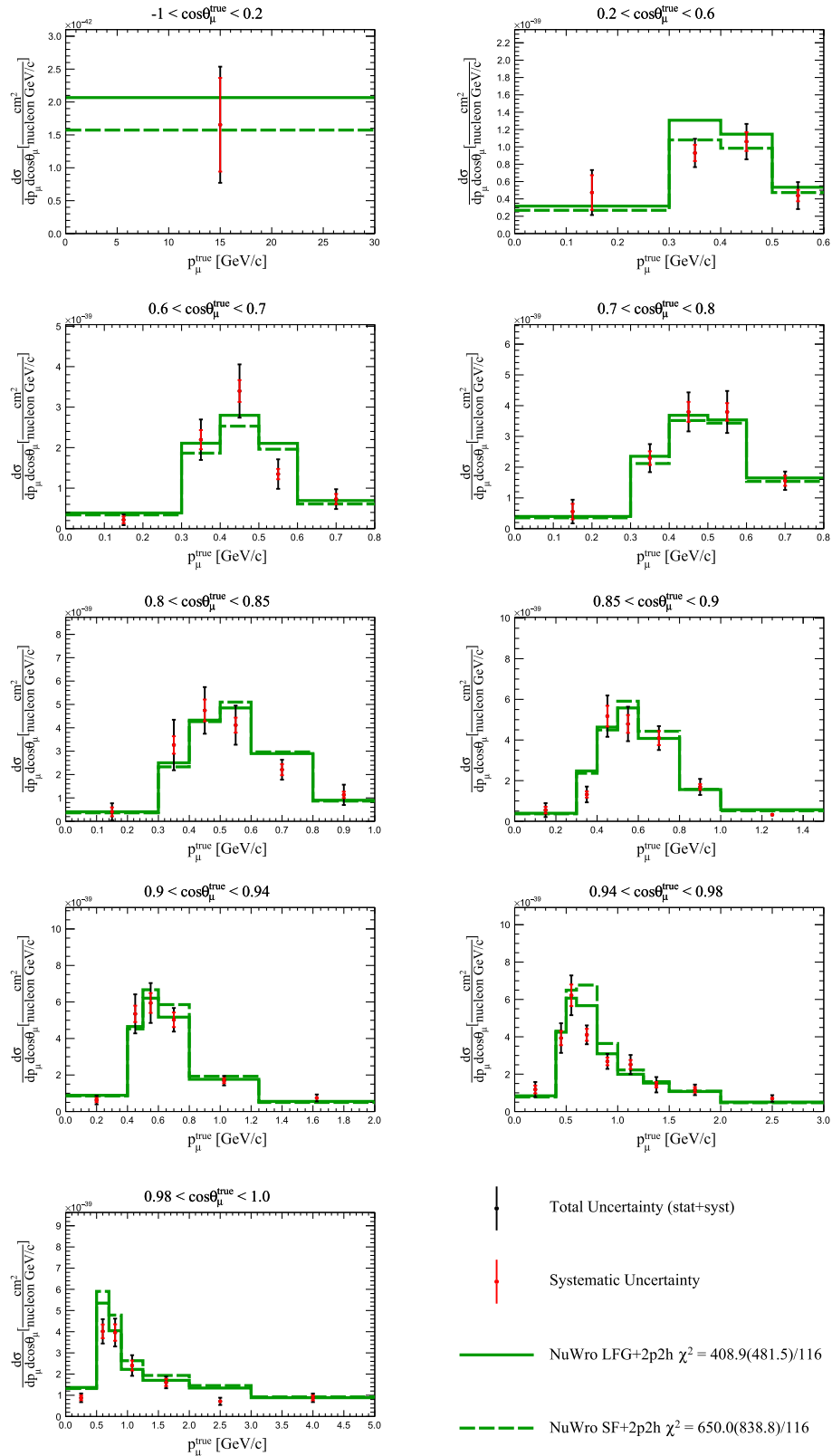
FIG. 31. Measured \bar{\nu}_\mu CC- 0\pi double-differential cross section per nucleon in bins of true muon kinematics with systematic uncertainty (red bars) and total (stat. + syst.) uncertainty (black bars). The result is compared with NUWRO version 18.02.1 with LFG + RPA (green solid line) and with the SF nuclear model (green dashed line), both including 2p2h predictions. The full and shape-only (in parenthesis) \chi^2 are reported. The last bin in momentum is not displayed for readability.
