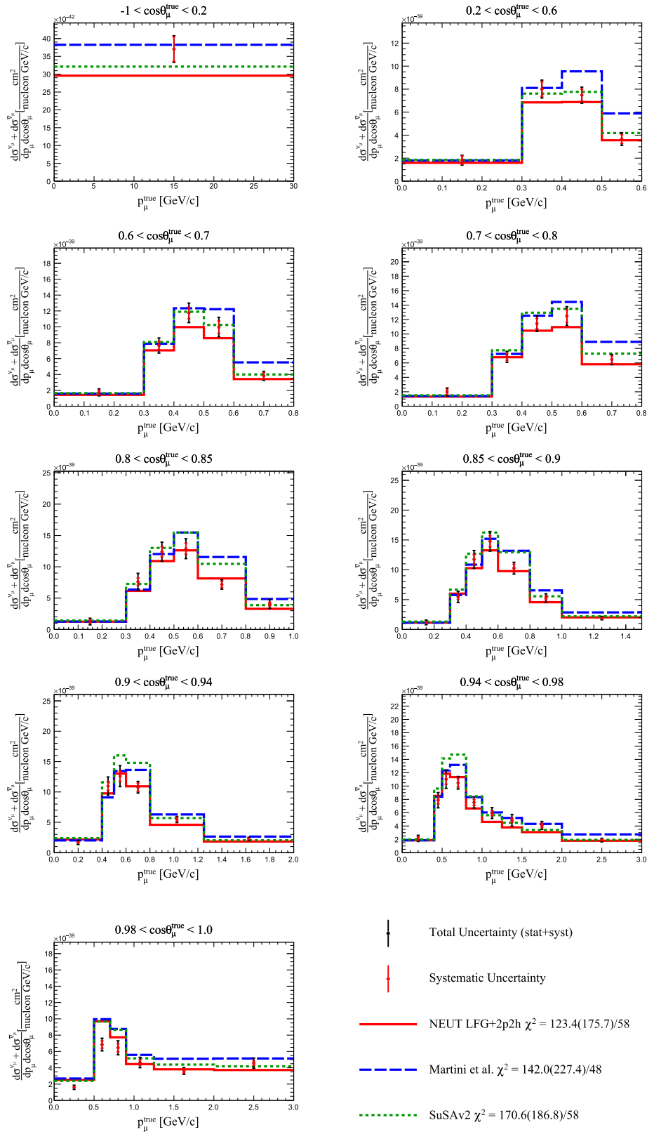
FIG. 22. Measured double-differential \nu_{\mu} + \bar{\nu}_{\mu} CC-0 \pi cross section sum in bins of true muon kinematics with systematic uncertainty (red bars) and total (stat. + syst.) uncertainty (black bars). The results are compared to NEUT version 5.4.1, which uses an LFG + RPA model with 2p2h (solid red line), Martini et al. (dashed blue line) and SUSAV2 (green dashed line) models. The full and shape-only (in parenthesis) \chi^2 are reported. The last bin in momentum is not displayed for readability.
