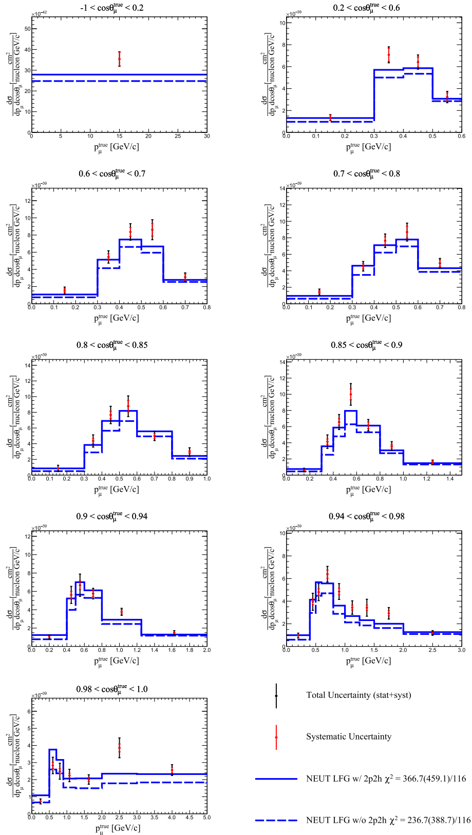
FIG. 15. Measured \nu_{\mu} CC- 0\pi double-differential cross section per nucleon in bins of true muon kinematics with systematic uncertainty (red bars) and total (stat. + syst.) uncertainty (black bars). The results are compared to NEUT version 5.4.1, which uses an LFG + RPA model, with (solid line) and without (dashed line) 2p2h. The full and shape-only (in parenthesis) \chi^2 are reported. The last bin in momentum is not displayed for readability.
