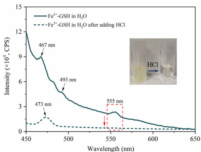
Figure 5 UV-Vis fluorescence spectra of the \text{Fe}^{3+} -GSH complex in deionised water with a concentration of 1.0 mg/mL, initial status (solid) and after adding 20 \mu\text{L} HCl (dash).
