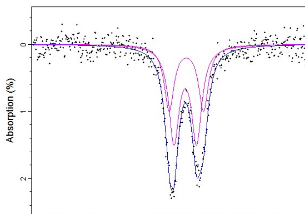
Figure 2 Fitted Mössbauer spectrum for the \text{Fe}^{3+} -GSH complex.
