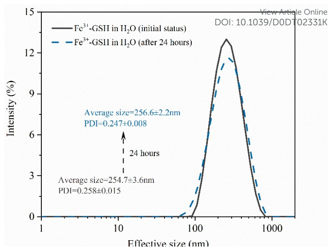
Figure 6 The effective size of \text{Fe}^{3+} -GSH in \text{H}_2\text{O} at a concentration of 0.5 mg/mL, initial status (solid) and storage in water for 24 hours (dash).
