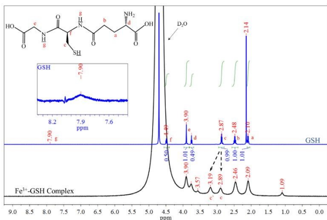
Figure 4 ^1\text{H} -NMR spectra of \text{Fe}^{3+} -GSH complex (black) and GSH (blue) in \text{D}_2\text{O} .
