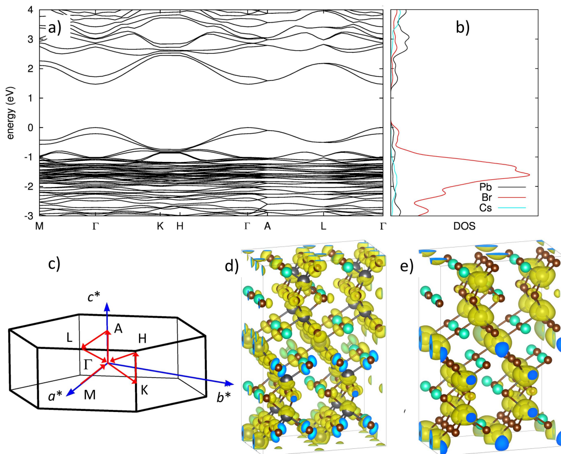
Figure 2. a) Band structure of 6H ‘APbBr 3 ’ perovskite (calculation with PBE xc-functional, including spin-orbit coupling, A = Cs); the valence band maximum is set to zero; b) corresponding partial density of states; c) first Brillouin zone for hexagonal primitive lattice; d-e) wavefunction localization of the valence band edge (d) and conduction band edge (e) at \Gamma point.
