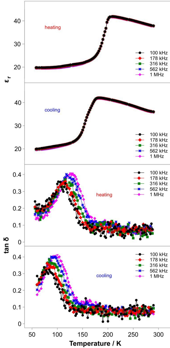
Figure 3. Temperature and frequency dependence of relative permittivity ( \epsilon_r ) and dielectric loss ( \tan \delta ) of \text{AzPbBr}_3 at the heating/cooling rate of 1 K/min.
