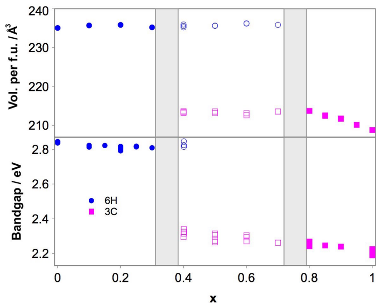
Figure 8. (Top) unit cell volume (expressed per ABX_3 formula unit (f.u.) for ease of comparison) and band gap (bottom) as a function of x for mixed cation compositions AZ_{1-x}MA_xPbBr_3 ( 0 \leq x \leq 1 ). Compositions with 0 \leq x \leq 0.3 and 0.8 \leq x \leq 1.0 form solid solutions with the 6H- and 3C-perovskite structures, respectively; a two-phase region forms for intermediate x . The grey regions represent the limits of each solid solution as determined by PXRD. Multiple data points at each value of x represent data for repeated sample syntheses.
