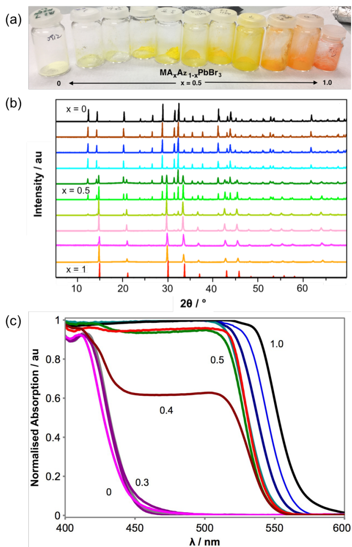
Figure 7. a) Color change of samples prepared according to composition \text{Az}_{1-x}\text{MA}_x\text{PbBr}_3 ( 0 \leq x \leq 1 ); b) PXRD data and c) absorption spectra as a function of x .
