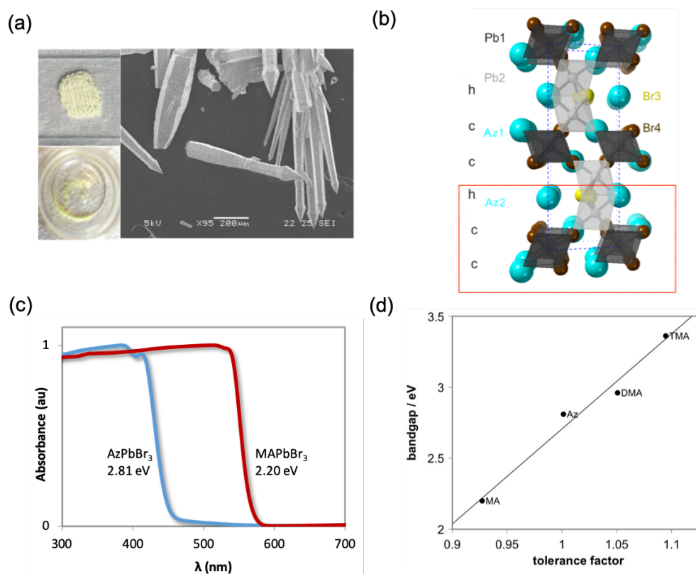
Figure 1. \text{AzPbBr}_3 : a) optical images of powder and single crystal \text{AzPbBr}_3 sample (left), and SEM micrograph of single crystals (right); b) 6H hexagonal perovskite structure as determined from single crystal XRD at 293 K (space group P6_3/mmc , lattice parameter a = 8.745 \text{ \AA} , c = 21.329 \text{ \AA} ) indicating (hcc)_2 packing sequence and combination of face- and corner-sharing octahedra; c) absorption spectra and associated band gap obtained from \text{AzPbBr}_3 and \text{MAPbBr}_3 powders. d) Dependence of band gap on tolerance factor for lead OIHP with different A-cations and resulting close packing of the perovskite structure adopted \text{MA}^+ (3C), \text{Az}^+ (6H), \text{DMA}^+ (4H) and \text{TMA}^+ (2H). 35,36,44
