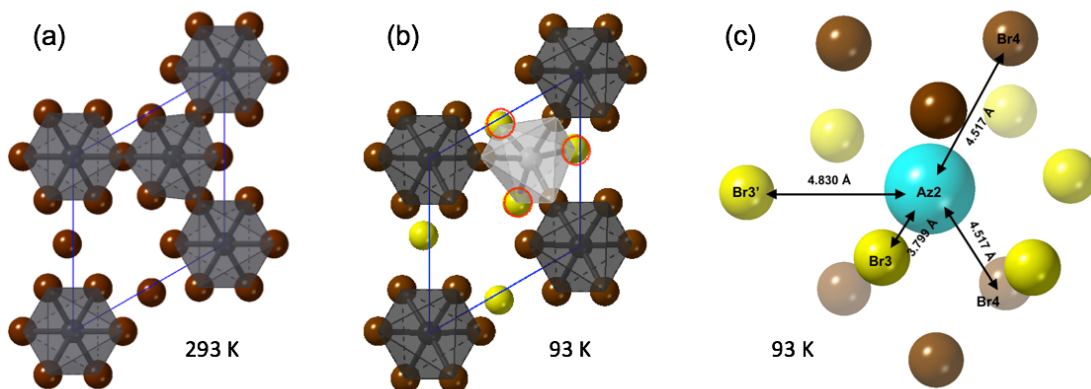
Figure 6. cch -fragment of the 6H AzPbBr 3 structure viewed down the c -axis at (a) 293 K and (b) 93 K, highlighting the distortion in the h layer (Br3 - yellow spheres) at 93 K compared to 293 K. (c) The resulting distortion of the dodecahedral environment occupied by the Az2 cation at 93 K.
