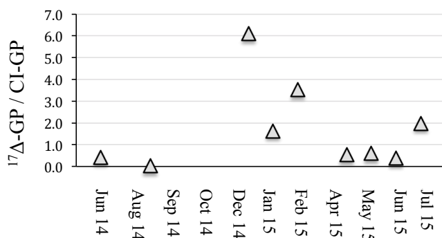
Figure 7. The relative difference between production rates obtained from mixed-layer model ( ^{17}\Delta -GP, following Luz and Barkan, 2000) and our whole column inventory approach (CI-GP).
