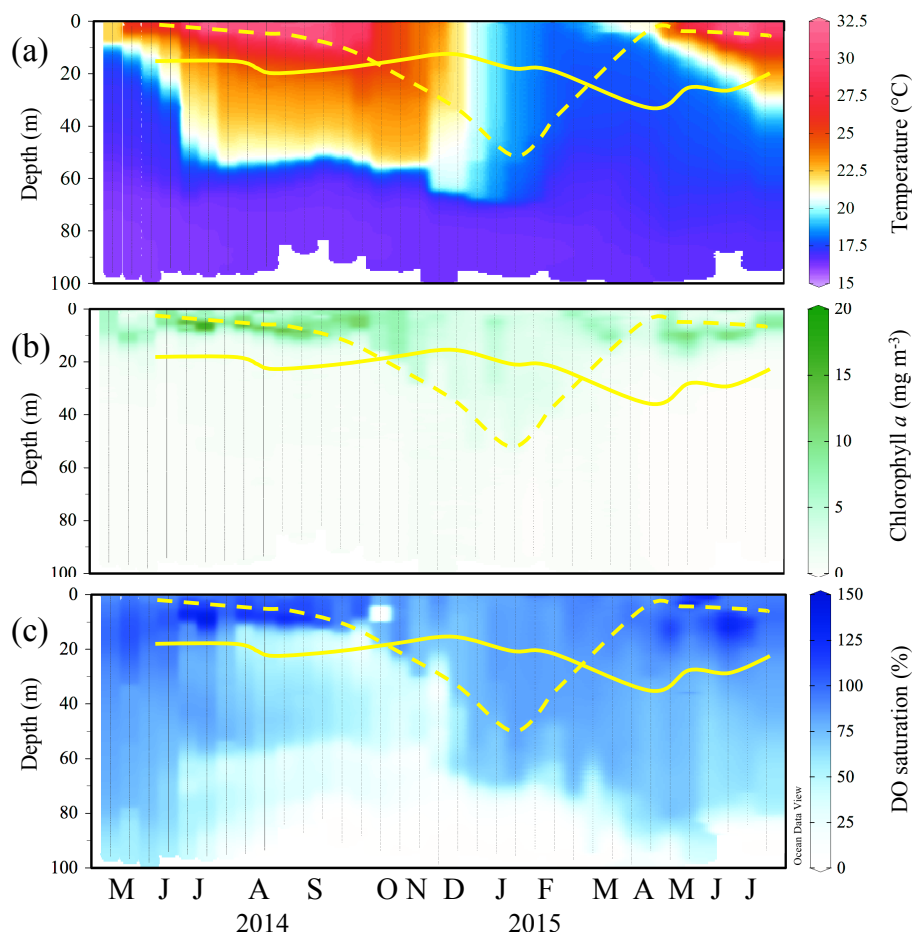
Figure 2. Seasonal variability in (a) temperature ( ^{\circ}\text{C} ), (b) chlorophyll a concentration ( \text{mg m}^{-3} ), and (c) dissolved oxygen saturation (%) from S1 in the Feitsui Reservoir (Fig. 1). Profile data were normally collected on weekly basis throughout the warmer months and every 2 weeks in winter. Solid yellow line indicates the limit of euphotic zone and dashed yellow line the depth of mixed layer.
