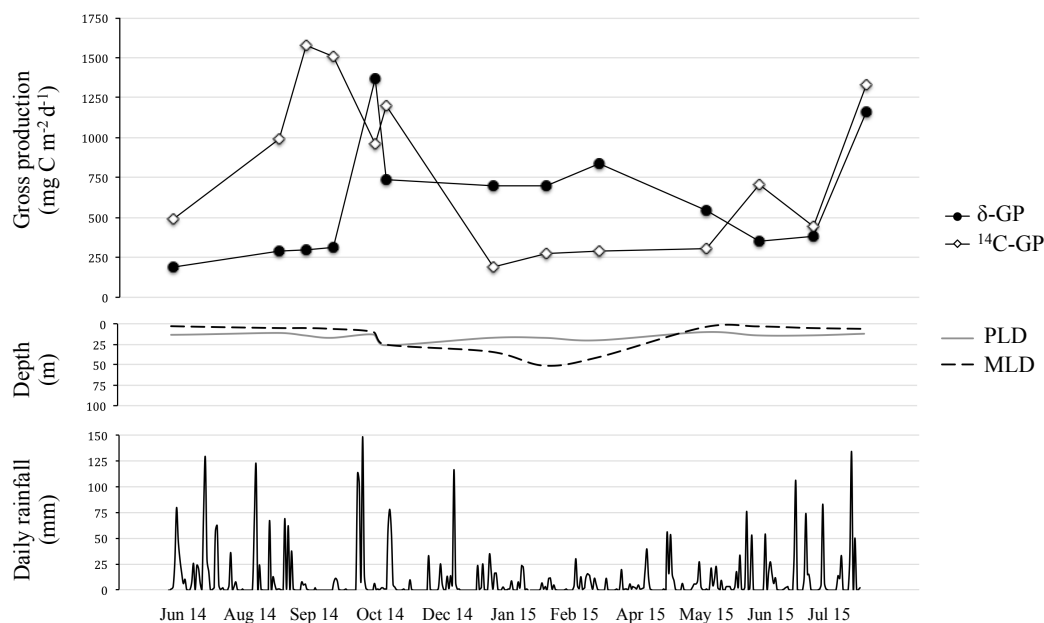
Figure 6. Comparison between dual-delta ( \delta -GP) estimates and ^{14}\text{C} -GP rates ( \text{mg C m}^{-2} \text{d}^{-1} ). PLD and MLD indicate photic layer depth and mixed-layer depth, respectively, and precipitation shows the total daily rainfall (mm).
