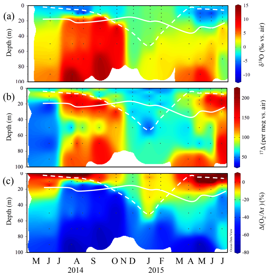
Figure 4. Seasonal variability in (a) \delta^{18}\text{O} of dissolved \text{O}_2 (‰ vs. air), (b) ^{17}\Delta (per meg vs. air), and (c) \Delta(\text{O}_2 / \text{Ar}) (%) in Feitsui Reservoir. Solid white line indicates the limit of euphotic zone and dashed white line shows the depth of mixed layer.
