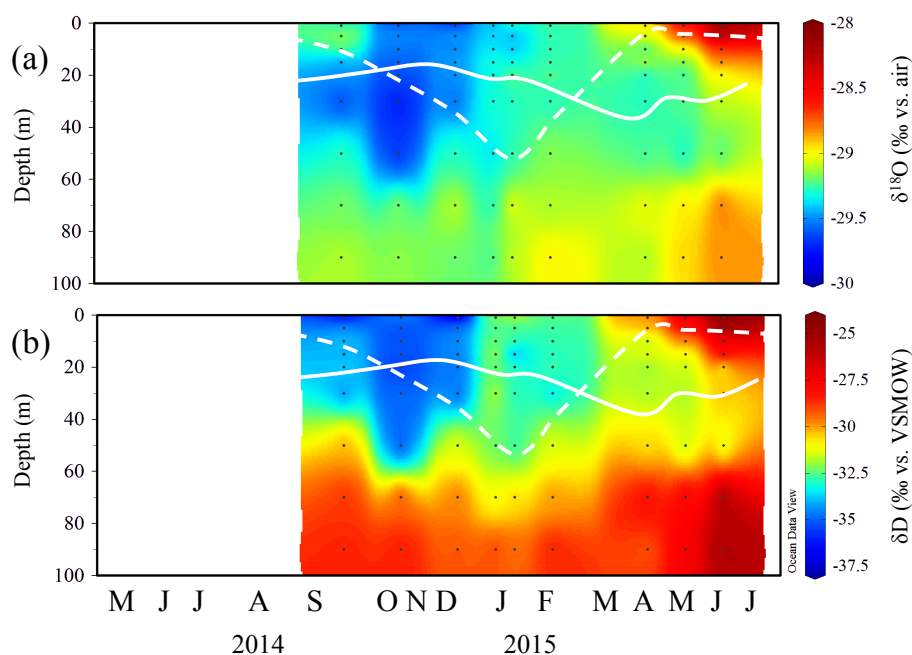
Figure 3. Seasonal variability in (a) \delta^{18}\text{O} of water \text{O}_2 (‰ vs. air) and (b) \delta\text{D} (‰ vs. VSMOW). Solid white line indicates the limit of euphotic zone and dashed white line the depth of mixed layer.
