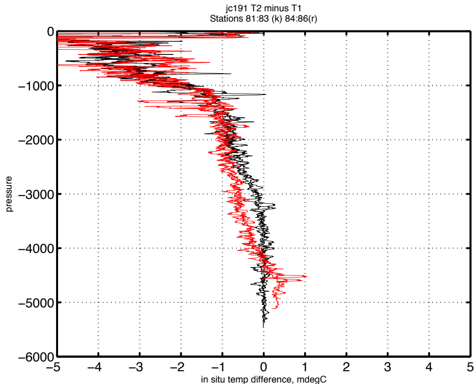
Figure 2.1: Sensor temperature differences. T22-T12 difference between CTD stations 81 to 83 (black line) and T22-T12 difference for CTD stations 84 to 86 (red line).
