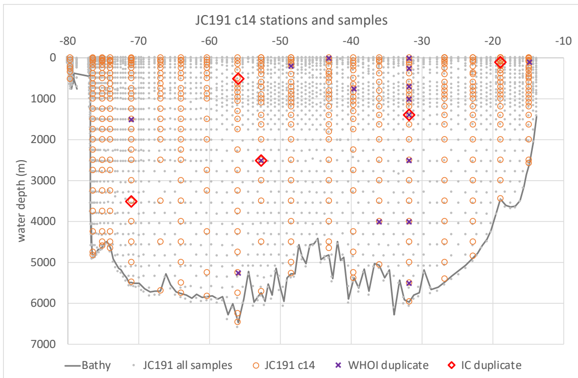
Figure 17.1: Locations of samples collected for radiocarbon analysis at the NERC Radiocarbon Facility (orange circles) and at NOSAMS (purple crosses). For reference, the locations of all CTD samples are shown in grey dots and the seabed is shown with a black line.
