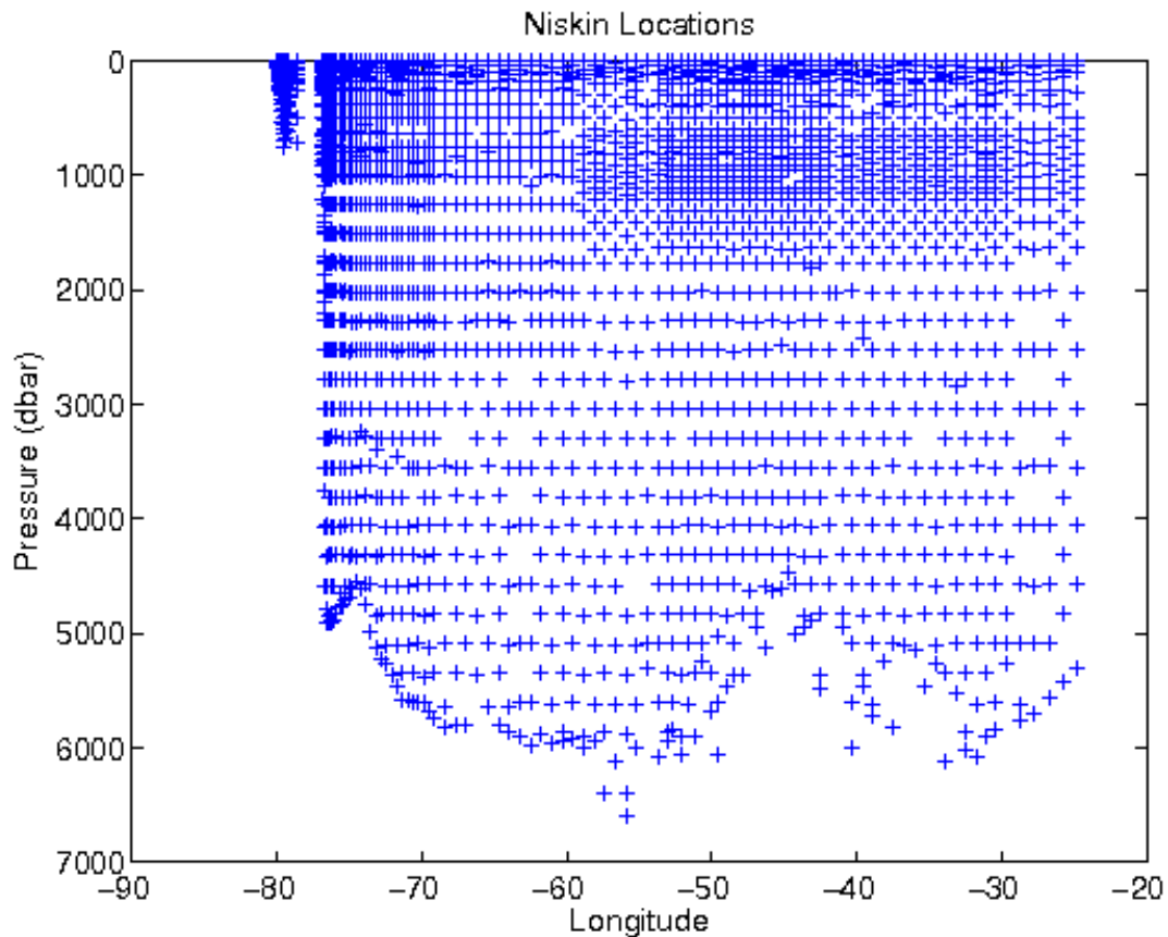
Figure 4.1: Cross section at 24° N of Niskin bottle depths where salts were drawn and analysed.
