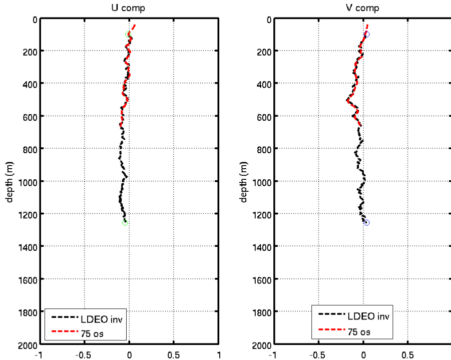
Figure 14.10: Post processed LDEO IX inverse u and v velocity components (dashed black line) constrained with SADCPCP (no GPS) and the 75os SADCPCP (red dashed line) for CTD station 063.
