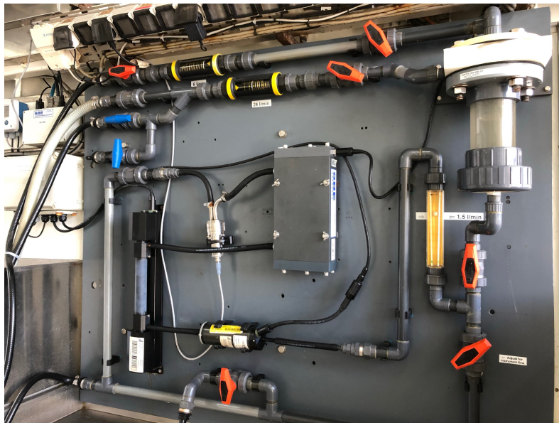
Figure 9.1: The underway instrumentation located in the bottle annex onboard the James Cook. The SBE45 TSG sensor can be seen in the middle of the board.
