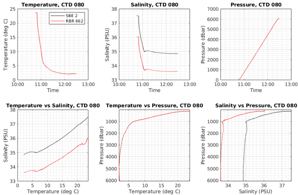
Figure 11.1: Downcast profiles of SBE 1Hz sensor 2 and RBR 662 for CTD 080, located at 24_N, 49_W. Top, left to right: timeseries of temperature (deg C), salinity (PSU) and pressure (dbar) are compared. Bottom, left to right: temperature against salinity, temperature against pressure and salinity against pressure.
