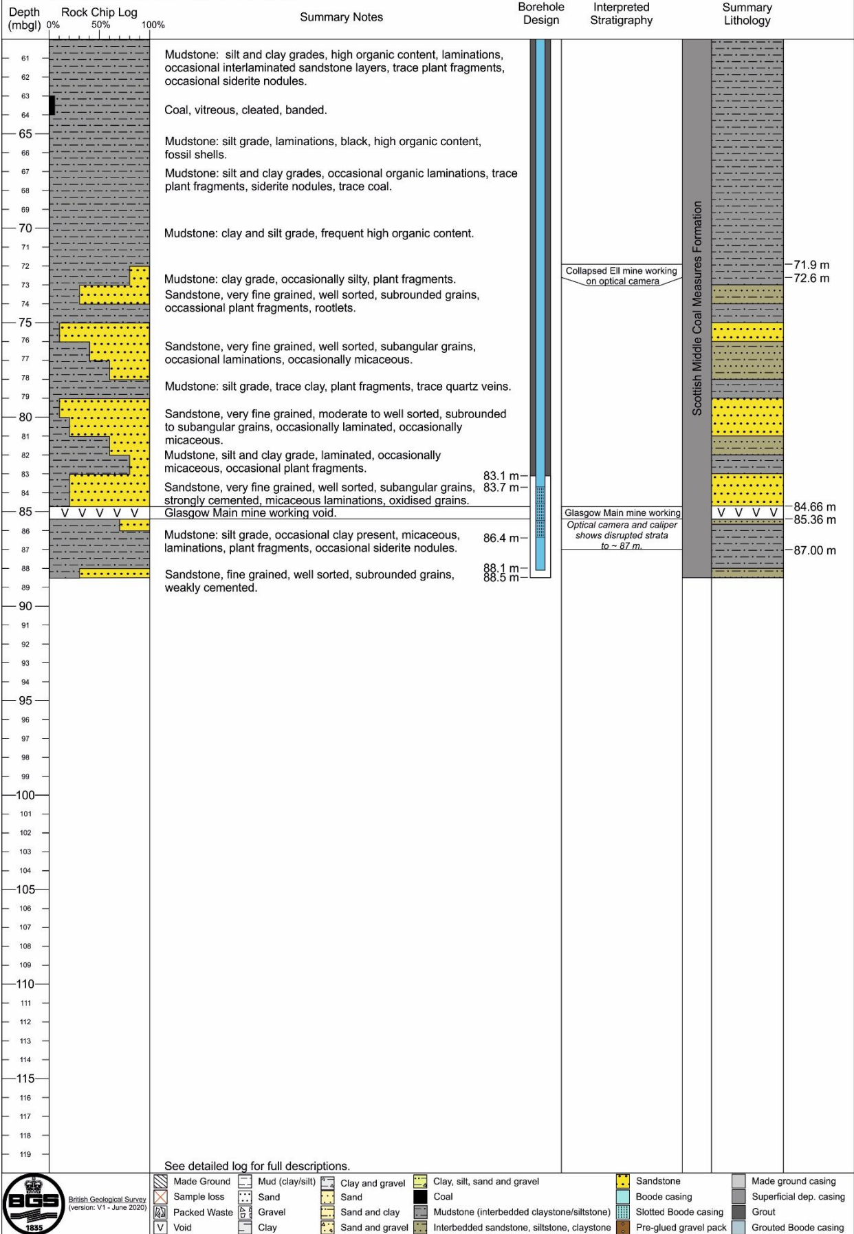
Figure 1 GGA05 summary log based on rock chip returns
