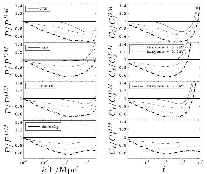
Figure 2. Left: combined feedback from baryons and massive neutrinos on the dark matter power spectrum, measured at z = 0 . Each panel shows the dark matter only model as the thick horizontal line, and the dark matter + baryons as the thin solid line. Top to bottom are AGN, REF, DBLIM and DM-ONLY baryon models, respectively. Also shown is the impact of neutrinos on each model, shown as thin dashed lines (0.2 eV), dotted lines (0.4 eV) and thick dash-dotted lines (0.6 eV). Right: same as the left-hand panel, but for the weak lensing power spectra, assuming the source redshift distribution given by equation (11).
