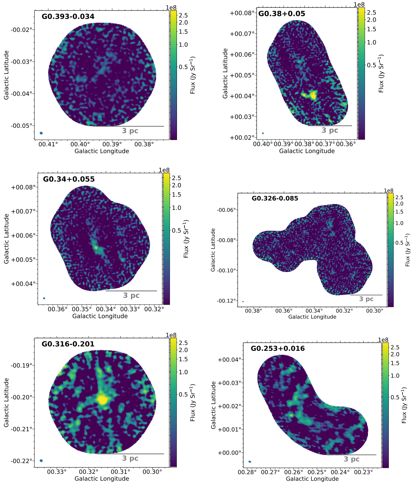
Figure 16. Images show the 1.3 mm dust continuum from the CMZoom Survey with a 3 pc scale-bar. The white contour shows the approximate 5- \sigma level while the black contour shows the approximate 10- \sigma level. All the images are displayed on same color scale from 2 - 290 MJy Sr -1 .
