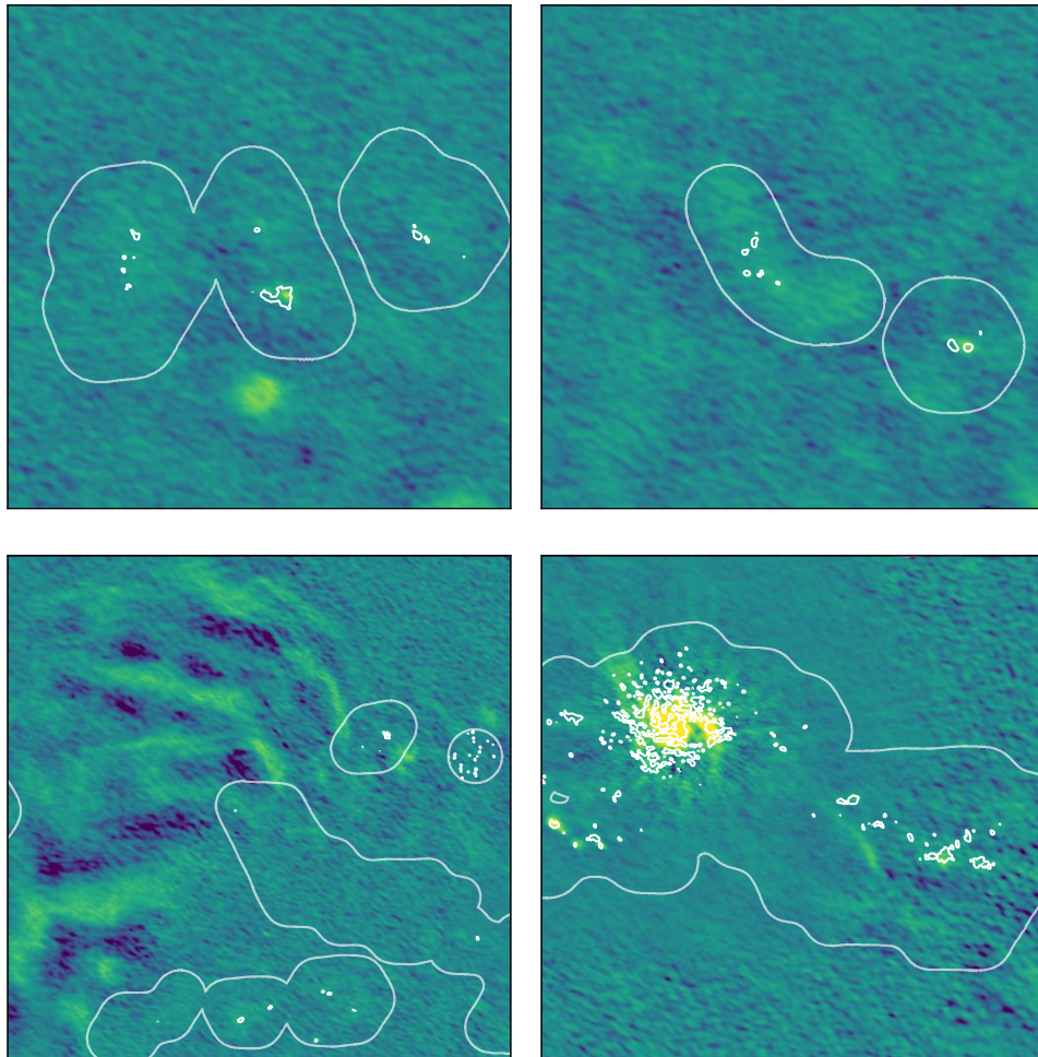
Figure 13. Comparison of CMZoom data with CARMA 3mm survey from Pound & Yusef-Zadeh (2018). All panels show the CARMA 3mm dust continuum 15+8 (Pound & Yusef-Zadeh 2018), which includes CARMA-15 (the 15-element array with six 10.4 m antennas and nine 6.1 m antennas) as well as CARMA-8 (the 8-element array of 3.5 m antennas) in the same colorscale. The CMZoom survey outline is shown in white. The bottom four figures show zoom-ins on several regions with 5\text{-}\sigma CMZoom contours (without primary beam correction) in white.
