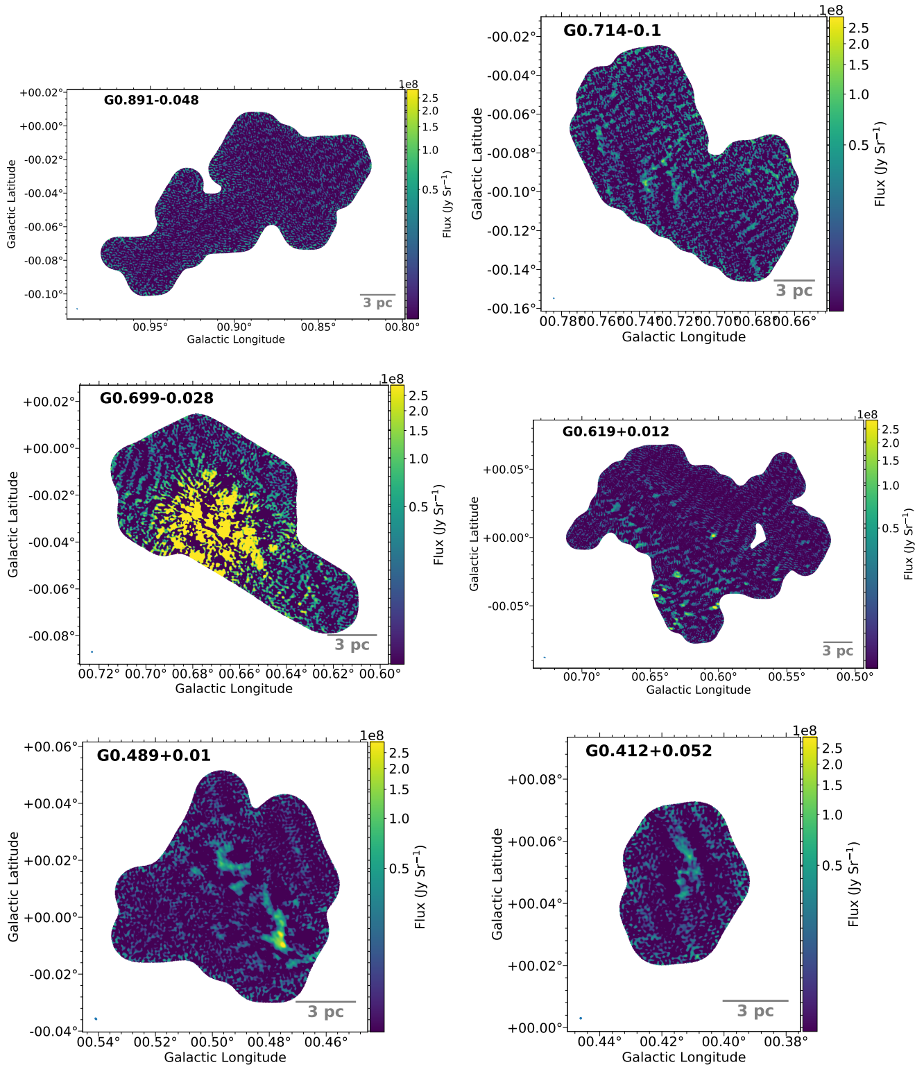
Figure 15. Images show the 1.3 mm dust continuum from the CMZoom Survey with a 3 pc scale-bar. The white contour shows the approximate 5- \sigma level while the black contour shows the approximate 10- \sigma level. All the images are displayed on same color scale from 2 - 290 MJy Sr -1 .
