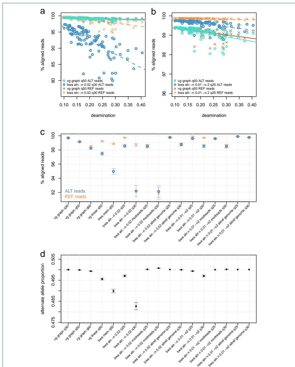
Figure 2: Comparing vg graph, bwa aln and bwa mem using simulated ancient DNA. Comparing bwa aln and vg map performance when aligning reads simulated from chromosome 11 of the Human Origins panel. Lines represent ordinary least squares (OLS) regression results for the allele/aligner conditions corresponding to their colors. a) Comparison between vg graph and bwa aln -n 0.02 . b) Comparison between vg graph and bwa aln -n 0.01 -o 2 . c) Comparison of the mean percentage (and 95% CI) of mapped reads in simulated data by vg graph , bwa aln and bwa mem using different alignment parameters and minimum mapping quality filtering thresholds. d) Mean alternate allele fraction (and 95% CI) of simulated reads after alignment with the different methods and minimum mapping quality filtering thresholds. We also show results obtained after processing simulated data with two previously published workflows for addressing reference bias: modified reads ('modreads') [10] and modified reference genome ('altref genome') [15].
