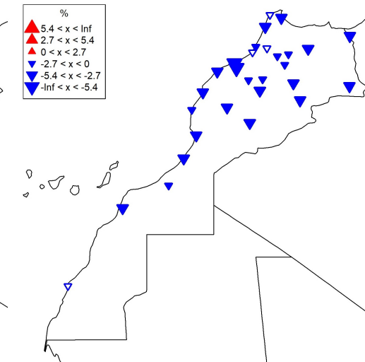
Figure 3: Trends in extreme temperature indices over Morocco for (a) warm days (NCMP4), (b) warm nights (Wnights) (c) cold days and (Cdays) and (d) cold night (NCMP5). The first column indicates trends at the national scale over the period 1984-2016 and the second column shows trends (per decade) at each individual station with varying record lengths from 1960 to 2016. The red and blue triangles indicate positive and negative trends respectively.
