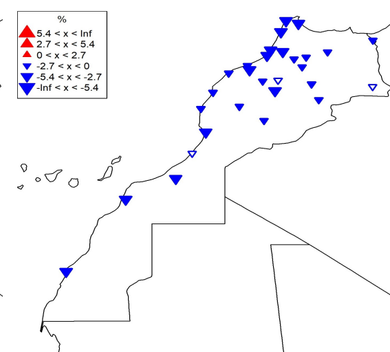
Figure 3: Trends in extreme temperature indices over Morocco for (a) warm days (NCMP4), (b) warm nights (Wnights) (c) cold days and (Cdays) and (d) cold night (NCMP5). The first column indicates trends at the national scale over the period 1984-2016 and the second column shows trends (per decade) at each individual station with varying record lengths from 1960 to 2016. The red and blue triangles indicate positive and negative trends respectively.
