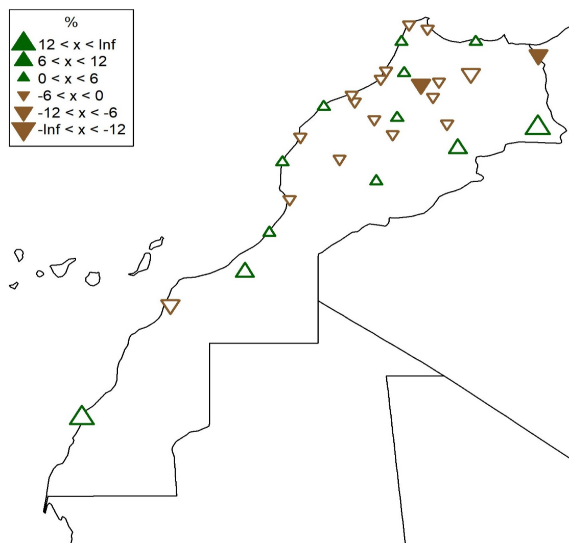
b) Total precipitation anomaly (NCMP2)
