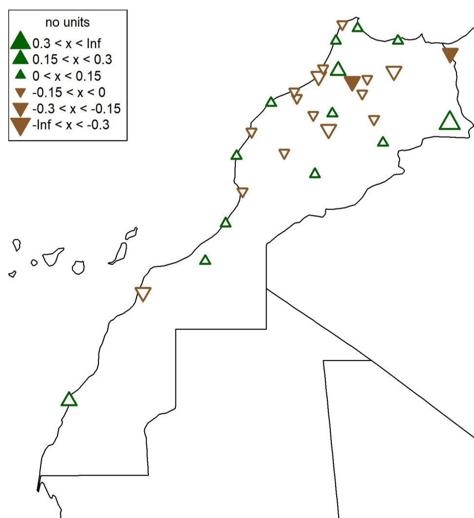
c) Standard Precipitation index (NCMP3)
