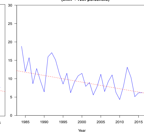
d) Cold nights (NCMP5)
