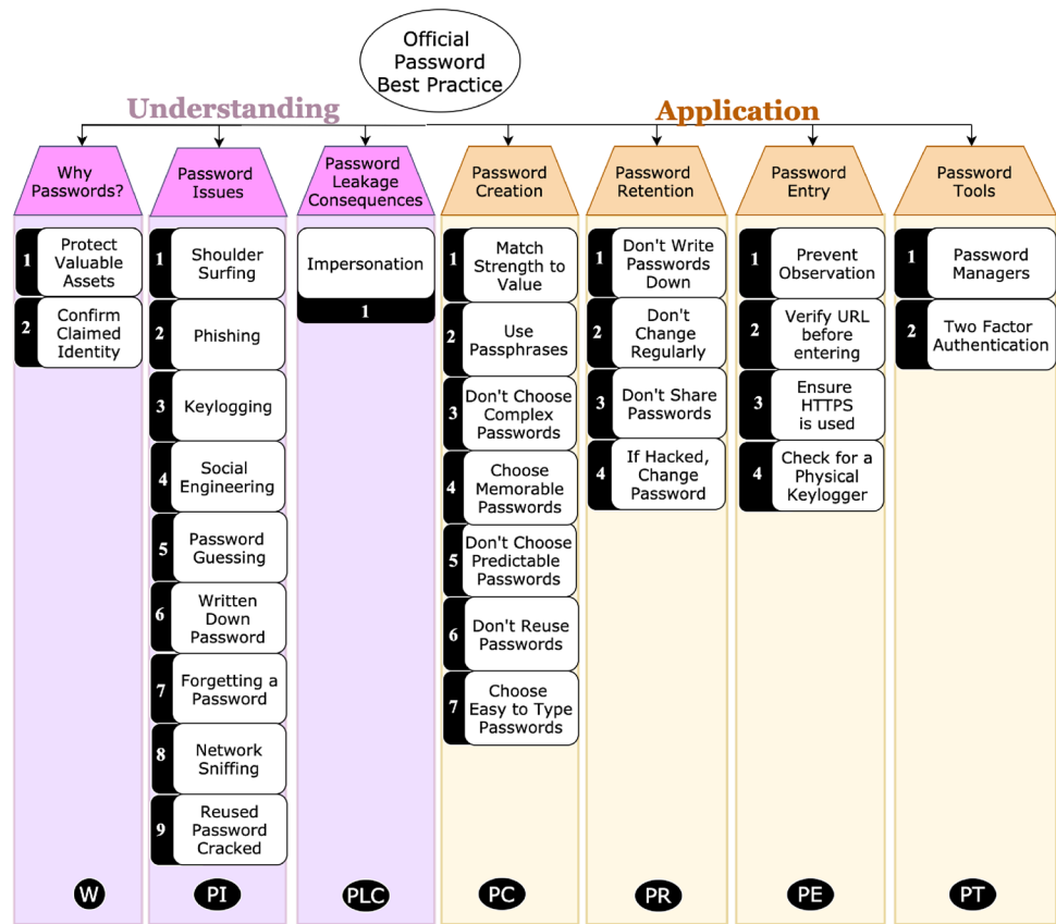
Fig. 2 Ontology of best practice password principles (amended from Prior and Renaud (2020))
