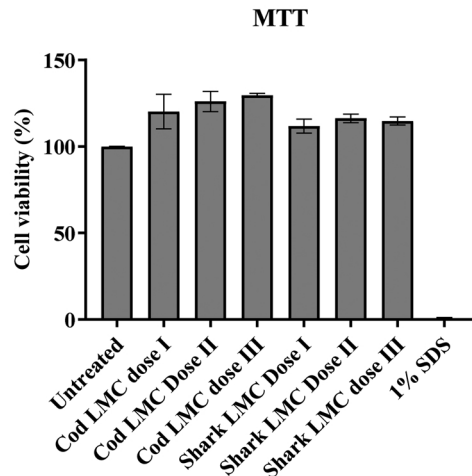
Fig. 5. Fish LMC modify the epithelial barrier properties. A. 16HBE140- cell monolayers were exposed apically to three doses of cod or shark LMC and TEER measured over time. TEER was normalized to untreated monolayers for each time point. Data show means with ranges (min to max) from three independent experiments performed in duplicates. B. Polarized monolayers were treated for 24 h with fish LMC (Dose III) and the permeability for FD10 was explored. Untreated cells were used as reference. n = 2 , data show mean \pm SD. C. Quantification of the PVs in basolateral cell culture medium after 24 h of apical stimulation in presence or absence of LMC. n = 3 , data show mean \pm SD. D. Cell viability analyzed by MTT assay 24 h after apical exposure to different doses of LMC. n = 3 , data show mean \pm SD. * p < 0.05 ; ** p < 0.01 ; *** p < 0.001 .
