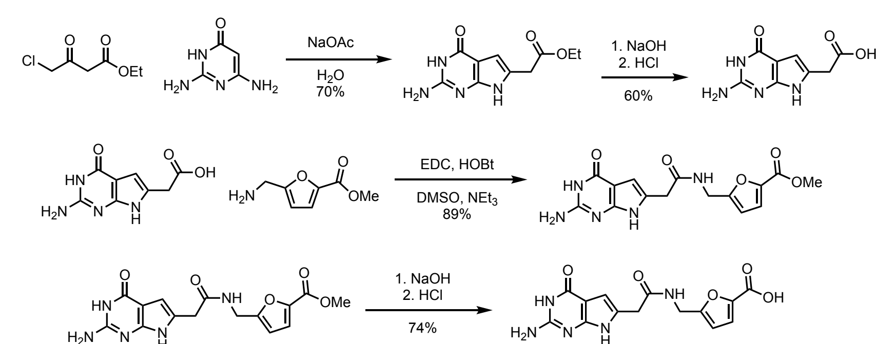
Figure 4. Synthesis of deazaguanine and with linker
