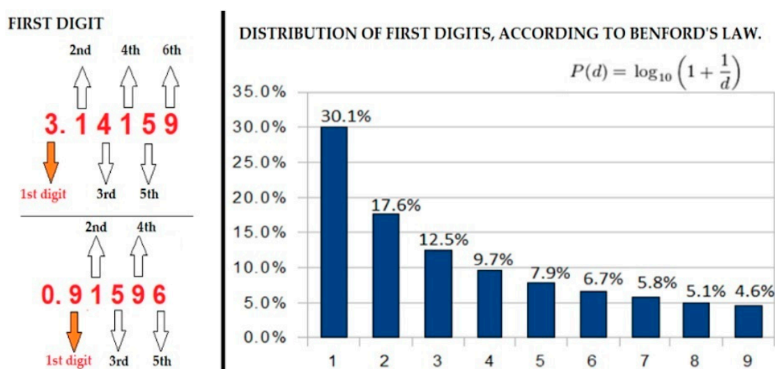
Figure 9. Distribution of first digits according to Benford’s law.
