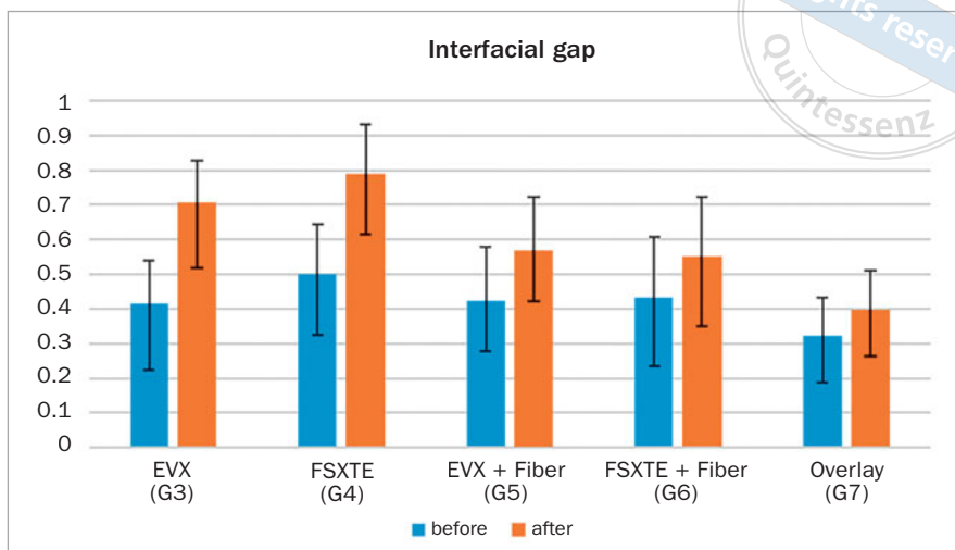
Fig 3 Mean interfacial gap of each group, expressed as mm 3 of volume, before and after fatigue loading in chewing simulator. EVX = everX Posterior; FSXTE = Filtek Supreme XTE; Fiber = everStickNET.
