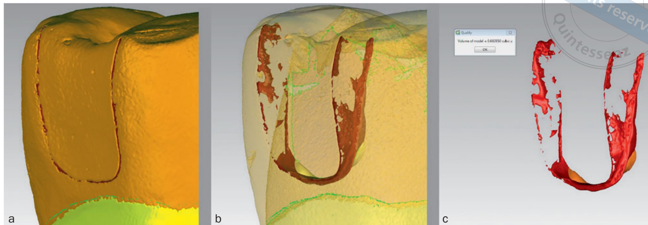
Fig 2 Micro-CT 3D images of specimens to calculate interfacial gap volume. a: Every specimen was 3D reconstructed dividing enamel, dentin, restoration, and voids using Hounsfield-scale spikes on Mimics software. Optimal quality STL images were then imported into Geomagic Quality for analysis. b: Same view with enamel, dentin, and restoration set to 60% transparency to better visualize void areas at the interface. c: Volume calculation was automatically performed by Geomagic Quality on void STL images, setting units in millimeters.
